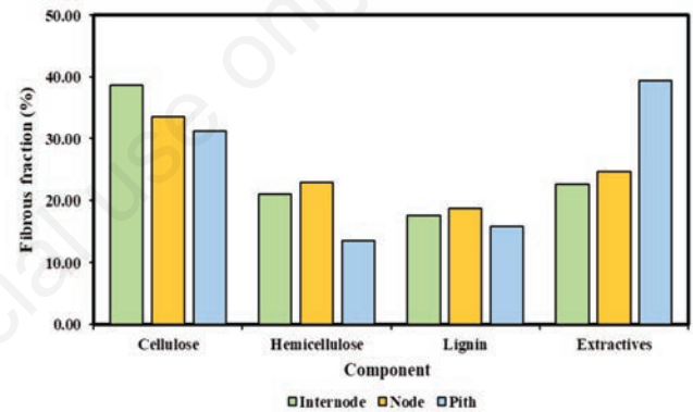
Figure 6. Results of the fibrous fraction analysis of the three components of vine shoots.
