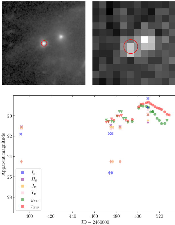
Figure 5. ZTF24aaueye. Top: 30 arcsec \times 30 arcsec Euclid I_E band image at JD = 2460509 and ZTF g-band discovery image at JD = 2460494; in both North on top and East to the left. Bottom: Light curve as in Fig. 4.
