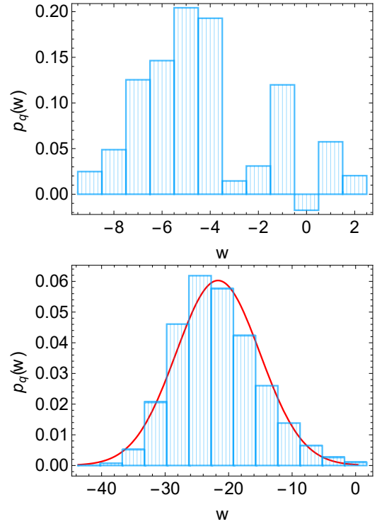
FIG. 2. The histogram of the work distribution. We put L = 10 in the top panel, L = 50 in the bottom panel, q = 1/2 , \beta = 1 , \lambda_\tau = 1.5 , \lambda_0 = 0.5 and \phi_k = \pi/4 . The red line corresponds to the Gaussian distribution probability in Eq. (38). We note that for L = 50 there is still some skewness. The histograms are calculated by using the characteristic function of Eq. (23).
