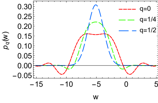
FIG. 1. The quasiprobability of work in Eq. (37) for different values of q . We put L = 50 , \beta = 1 , \lambda_0 = 0.9 , \lambda_\tau = 1.1 and \phi_k = 0 .
