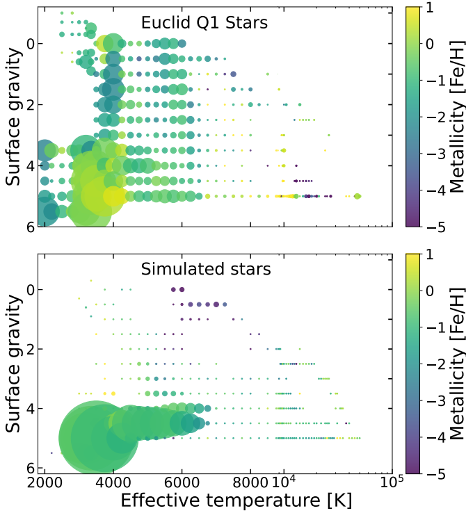
Fig. 18. Logarithmic surface gravity as a function of effective temperature for star-classified objects, as obtained from the Phosphoros best-fit SED (top panel) and for stars from the Euclid simulated catalogue in the EDFs (bottom panel). Colours of points are related to the mean stellar metallicity, while the size of the points is proportional to the number of objects.
