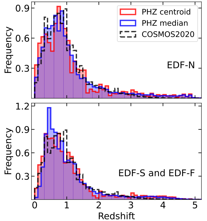
Fig. 11. Redshift distribution for VIS-detected I_E < 24.5 objects from the EDF-N (top panel), and from the EDF-S and EDF-F (bottom panel). We use as redshift estimate the median of the z PDFs (blue histograms) and the centroid of the main peak (red histograms). Dashed histograms are obtained from the COSMOS2020 catalogue.
