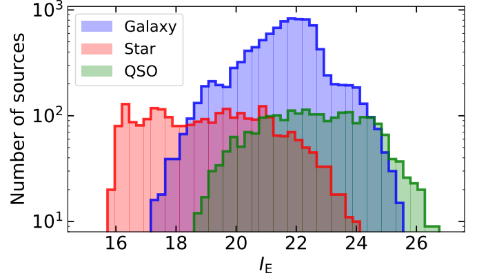
Fig. 2. I_E magnitude distribution per class of objects in the training sample for classification.
