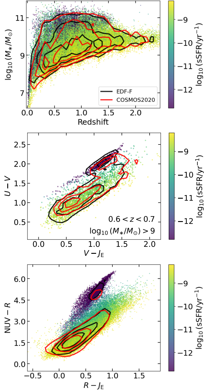
Fig. 16. Scatter plots of the EDF-F galaxies without the problematic population, colour-coded by \log_{10}(\text{sSFR}/\text{yr}^{-1}) (for visual reason, only 10% of the sources are plotted). Contour plots are for the EDF-F galaxies (black lines) and for the COSMOS2020 sample (red lines). Top: Stellar mass as a function of redshift. Central: U - V versus V - J_E in a limited range of z and M_* , as reported in the panel. Bottom: \text{NUV} - R versus R - J_E .
