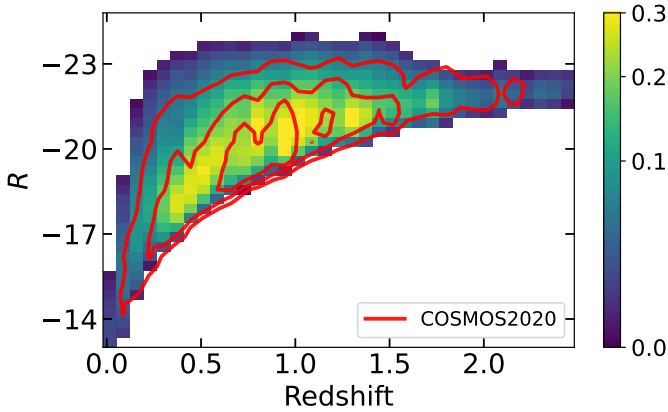
Fig. 15. Density plot of R -band absolute magnitude as a function of redshift for the EDF-F galaxies (excluding the problematic galaxy population). Density contours from the COSMOS2020 catalogue are superimposed.
