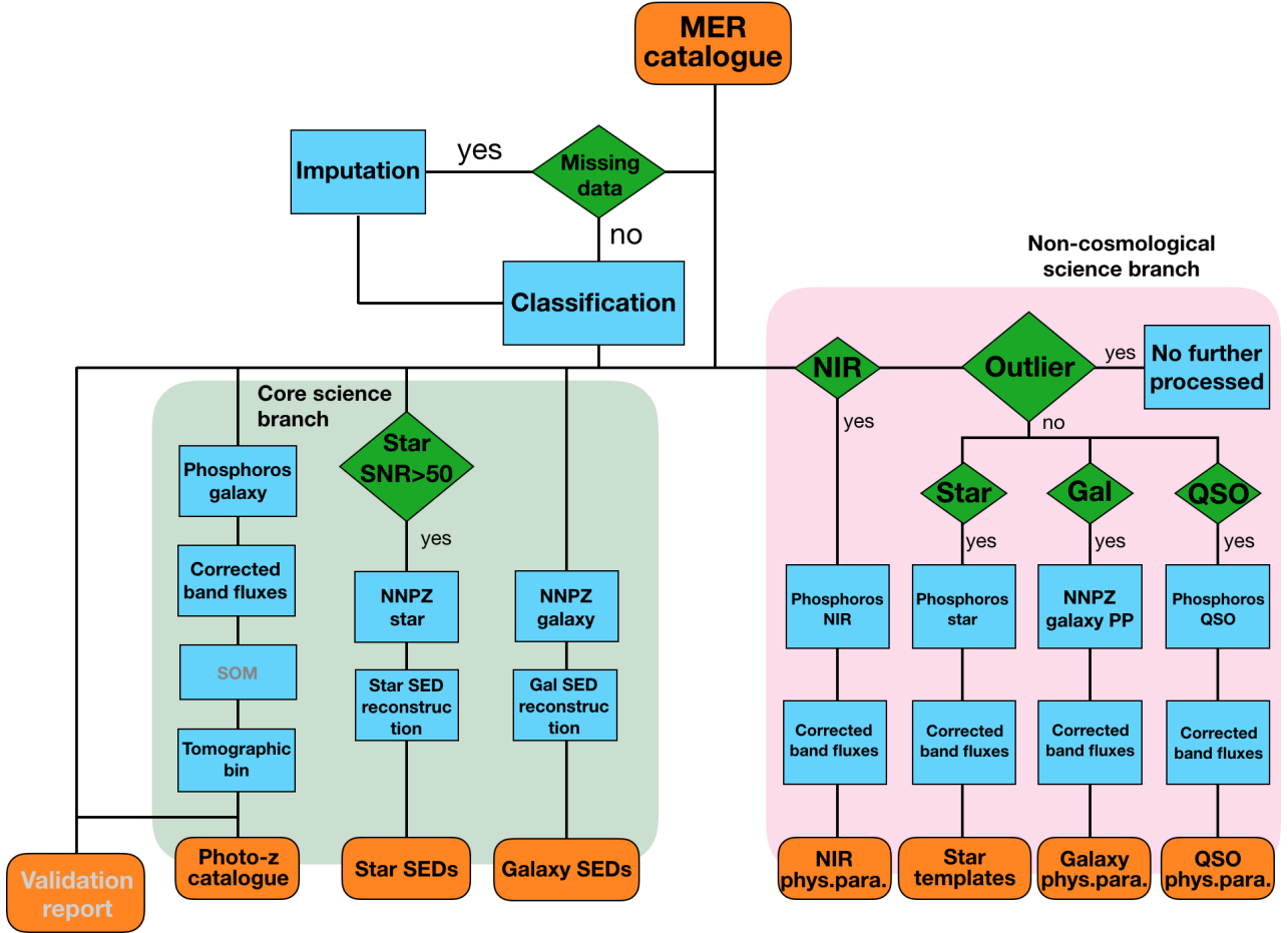
Fig. 1. Diagram of the production pipeline for the Q1 release. Orange boxes are for input or output products, green diamonds for conditional statements, and blue boxes for specific tasks. In grey, it shows all the steps of the pipeline that have been performed, but whose products are not included in the public release.
