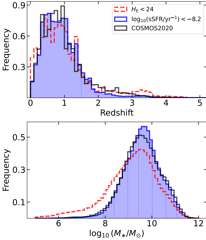
Fig. 14. Redshift (top panel) and stellar mass (bottom panel) distribution for galaxy-classified objects in the EDF-F with \log_{10}(\text{sSFR}/\text{yr}^{-1}) < -8.2 , compared with the distributions from the COSMOS2020 catalogue (black lines). The red dashed histograms are for all EDF-F sources with H_E < 24 .
