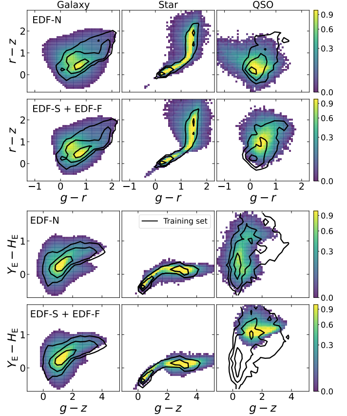
Fig. 5. Two-colour density plots for the different types of objects in the northern and southern tiles, compared with the training set (black contour curves). Colours are corrected for Galactic extinction, as described in Appendix A.1.
