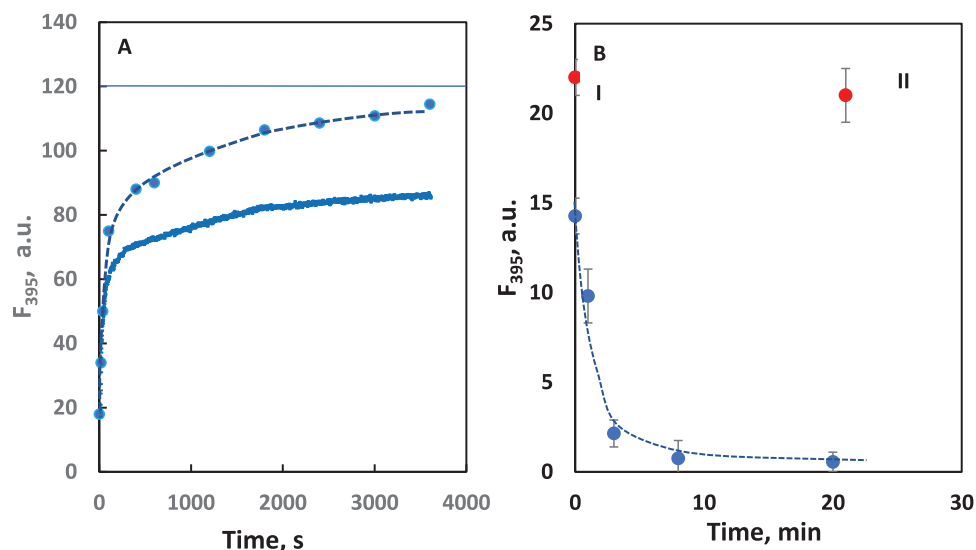
Figure 7. A) Kinetic of the exchange process between amine Py-C 1 NH 2 and 1 using AuNPs treated with NaBH 4 (blue circles). The dashed line represents the fitting of the two kinetic processes. The horizontal line at F_{395} = 120 represents the maximum fluorescence obtained by addition of thiol C 8 SH. For comparison, the exchange kinetics of the same amines but using AuNPs not treated with NaBH 4 is reported. The conditions are the same as those of Figure 3A. B) Fluorescence observed in solutions obtained after the addition of an excess of amine 1 to the GC electrode modified with the AuNPs passivated with 1.6 \mu\text{M} Py-C 1 NH 2 following increasing oxidation times (conditions: 1.1 V vs Ag/AgCl, CH 3 CN, 0.1 M TBAPF 6 ). The red points indicated with I and II represent the fluorescence measured for solutions collected at time 0 (I) and 20 min (II) upon addition of thiol C 8 SH. Each point represents a different experiment. The experiments were run in duplicate. The dashed line was drawn to guide the eye.
