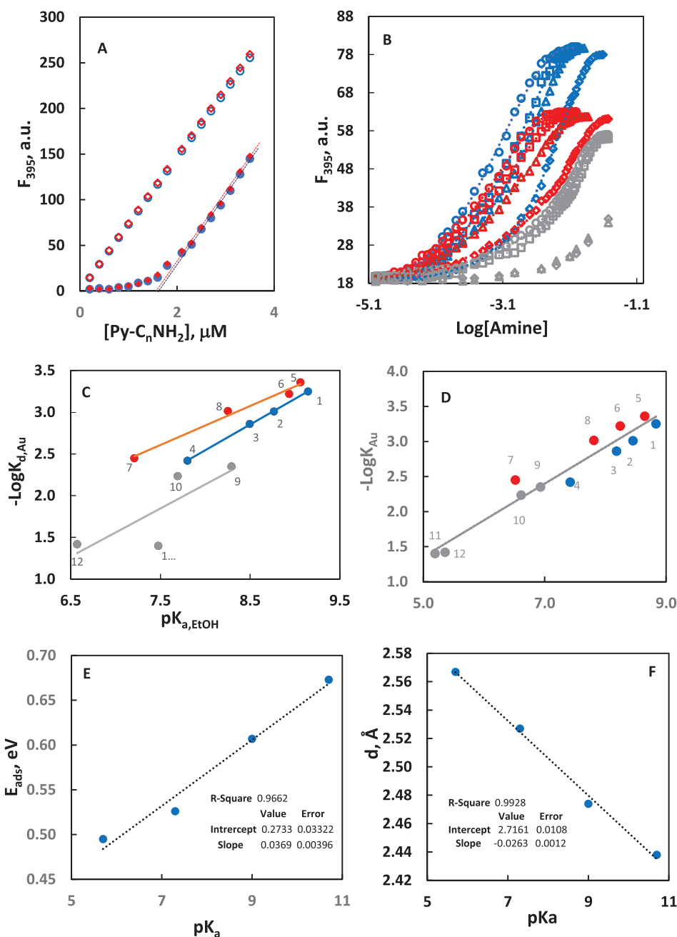
Figure 2. A) Fluorescence intensity (395 nm) as a function of the concentration of added amines Py-C 1 NH 2 (red diamonds) and Py-C 8 NH 2 (blue circles) to ethanol (empty symbols) and to a solution of nanoparticles (filled symbols). The intersection between the two straight lines was taken as the surface saturation concentration (SSC). Conditions: 35 °C, EtOH, [AuNPs] = 8.6 nm. B) Binding isotherms obtained by following the F_{395} upon addition of increasing amounts of amines 1–12. In blue: primary amines, red, secondary, gray, tertiary. Circles: amines 1, 5, 9; squares: amines 2, 6, 10; triangles: amines 3, 8, 12; diamonds: amines 4, 7, 11. Conditions as for panel (A). C) Log plot of the pKa in ethanol of the amines and their apparent dissociation constant for the gold surface obtained by interpolation of the data of (B). Data were fitted by linear regression analysis. For amines 11 and 12 F_{max} was arbitrarily set at the value of that obtained for amine 9. Errors for affinity constants (two independent measurements) are \pm 5\% for amines 1, 2, 5, 6, 8; \pm 7\% for amines 3, 4, 7, 9, 10; and \pm 15\% for amines 11 and 12. D) Log plot of the pKa in ethanol of the amines corrected for the steric hindrance parameter E_s (see Table 1) and their apparent dissociation constant for the gold surface obtained by interpolation of the data of (B). Data were fitted by linear regression analysis. All other conditions were identical to those of (C). E) Adsorption energies ( E_{ads} , eV) calculated for amines NH 2 CH 2 CH 3 , NH 2 CH 2 CH 2 F, NH 2 CH 2 CHF 2 , NH 2 CH 2 CF 3 on Au(111) surfaces plotted against their pKa. F) Measure of the N–Au distance ( d ) for the four amines from the Au atom of the (111) surface as a function of their pKa. For both panels (D) and (E), the red lines were obtained through a linear regression fit of the data; fitting parameters are contained within the inset tables of each panel.
