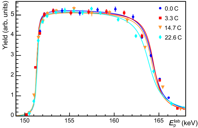
FIG. 3. Thick-target yield curve of the E_R^{\text{lab}} = 151 keV resonance illustrating the target thickness, and change of target profile with increasing accumulated charge. The fitted curves are shown to guide the eye.
