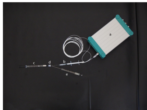
Fig. 2. Microfibre optic oxygen meter, Microx TX3 (A), equipped with a needle type optical microsensor (B); gas-tight Hamilton syringe containing the sample (C) and sealed with a silicon pierceable cap (D); (E) Hamilton syringe used to inject FCCP during oxygen measurement by piercing the silicon cap (D).
