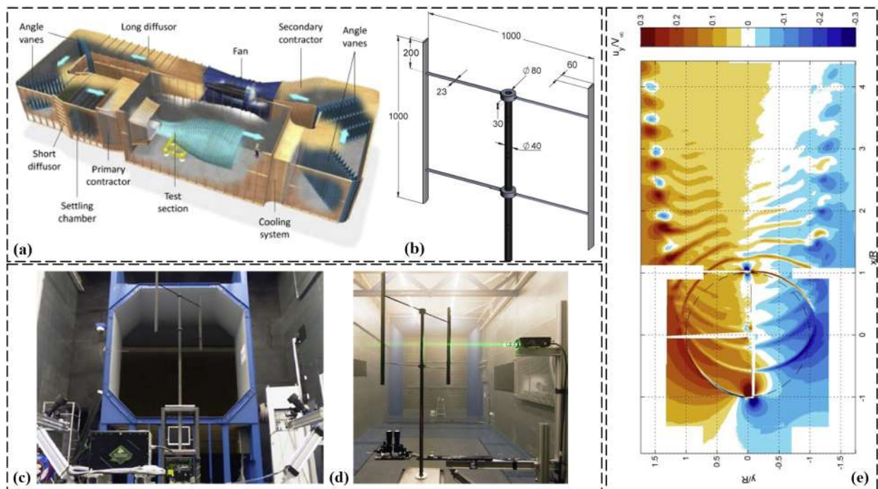
Figure 23. Stereoscopic particle image velocimetry. (a) Schematic of the TUDelft Open Jet Facility (reproduced with permission from Tescione, Renewable Energy , published by ELSEVIER, 2014 [87]). (b) Wind turbine model (dimensions in mm) (reproduced with permission from Tescione, Renewable Energy , published by ELSEVIER, 2014 [87]). (c) Stereoscopic PIV configuration (reproduced with permission from Tescione, Renewable Energy , published by ELSEVIER, 2014 [87]). (d) Planar PIV configuration (reproduced with permission from Tescione, Renewable Energy , published by ELSEVIER, 2014 [87]). (e) Contours of normalized out of plane vorticity for the combined field of views of the horizontal plane (reproduced with permission from Tescione, Renewable Energy , published by ELSEVIER, 2014 [87]).
