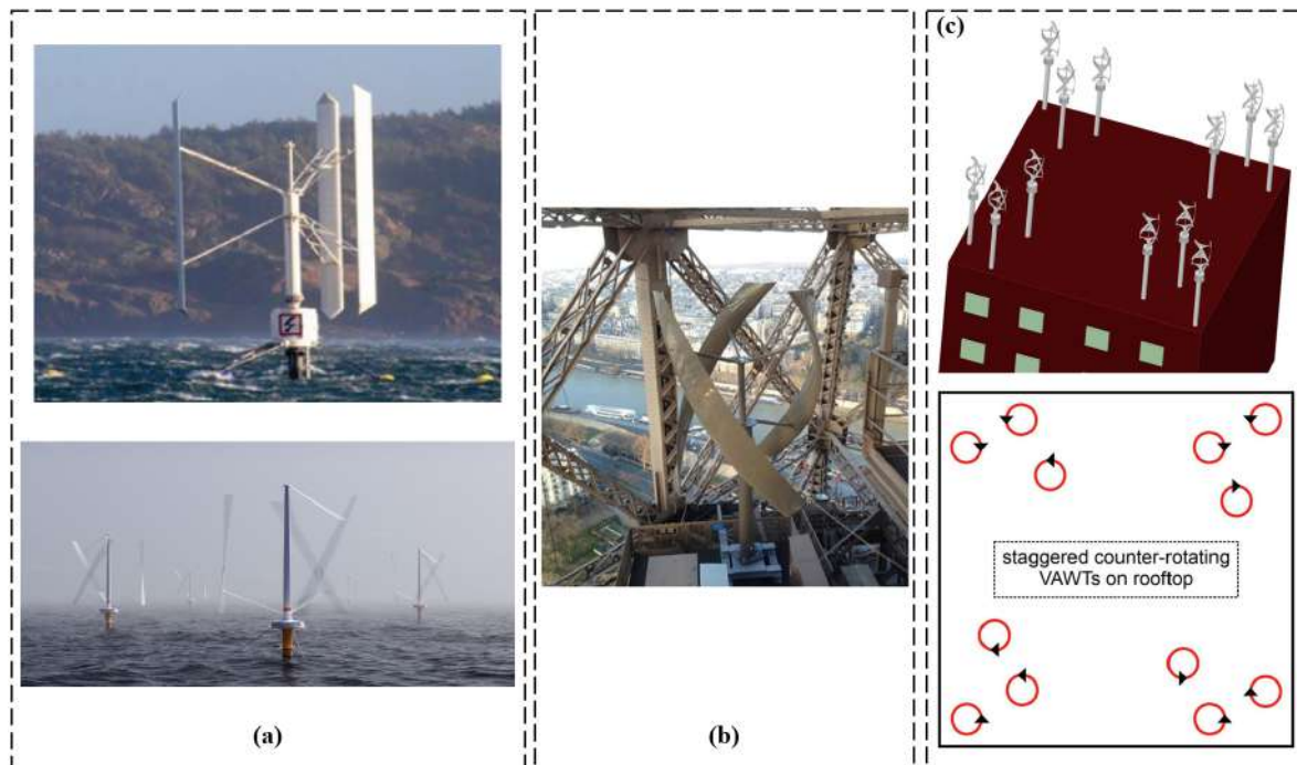
Figure 4. (a) S1 30 kW working prototype (reproduced with permission from Martin Rosander, Case Study: SeaTwirl—The Future of Offshore Floating Wind Turbines , published by ANSYS, Inc, 2018 [3]), (b) application of wind energy in urban areas (VAWT applied in the Eiffel Tower, France) (reproduced with permission from Ye Li, Energy Conversion and Management , published by ELSEVIER, 2021 [4]), and (c) schematic of 12 Darrieus helical VAWTs installed in a staggered arrangement on a rooftop. Each pair of adjacent turbines is counter-rotating (reproduced with permission from Rezaeiha, Energy Conversion and Management , published by ELSEVIER, 2020 [5]).
