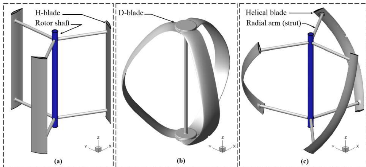
Figure 3. (a) H-Darrieus wind turbine, (b) D-Darrieus wind turbine, and (c) Helical-Darrieus wind turbine.
