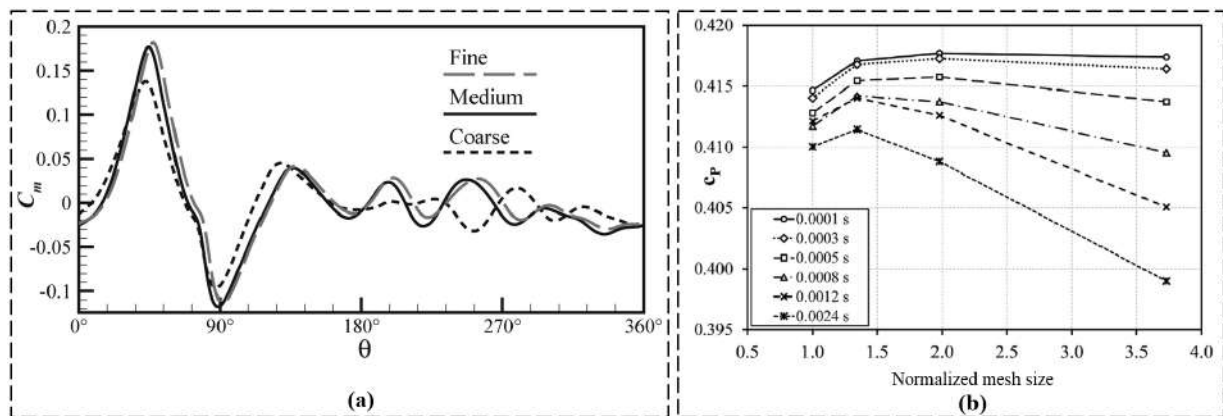
Figure 7. (a) The variations in the torque coefficient for one blade, as a function of Darrieus angular position, for the three grid resolutions at TSR=1.0 (reproduced with permission from Arab, Renewable Energy , published by ELSEVIER, 2017 [24]). (b) Sensitivity analysis at \lambda = 3.3 : power coefficient ( C_p ) as a function of the normalized mesh size (reproduced with permission from Ferrari, Energy , published by ELSEVIER, 2016 [48]).
