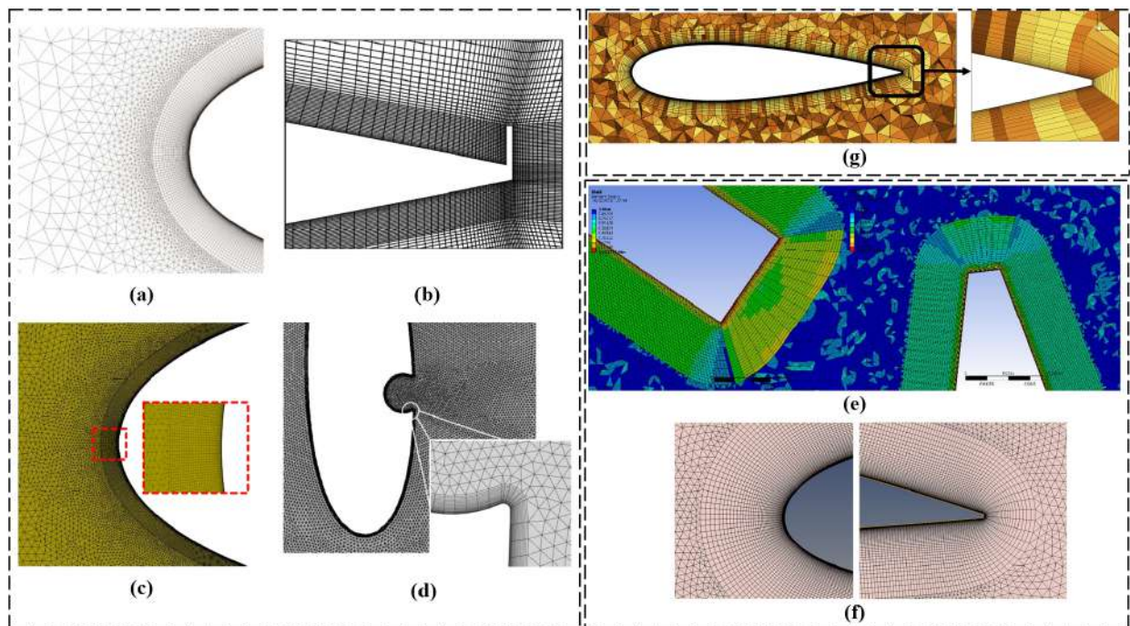
Figure 9. (a) Representation of the mesh near the blade walls and for the rotating domain (hybrid mesh near the airfoil leading edge) (reproduced with permission from Bedon, Renewable Energy , published by ELSEVIER, 2016 [43]), (b) mesh distribution of the airfoil with GF (reproduced with permission from Ni, Energy , published by ELSEVIER, 2021 [71]), (c) computational grid (near wall grid resolution) (reproduced with permission from Hand, Computers & Fluids , published by ELSEVIER, 2017 [23]), (d) generation of the boundary layer on the blade wall (reproduced with permission from Sobhani, Energy , published by ELSEVIER, 2017 [58]), (e) the worst elements of the hybrid grid structure lied on the tips of the blades (reproduced with permission from Hosseini, Energy conversion and management , published by ELSEVIER, 2019 [72]), (f) mesh details of the fourth grid (G4)—Mesh sensitivity analysis (reproduced with permission from Balduzzi, Renewable Energy , published by ELSEVIER, 2016 [22]), and (g) structured grid close to the turbine blade (reproduced with permission from Karimian, Energy , published by ELSEVIER, 2020 [18]).
