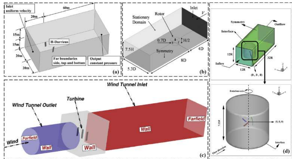
Figure 12. (a) Computational domain, including boundary conditions (non-scaled) and the grid computational domain (reproduced with permission from Joo, Energy , published by ELSEVIER, 2015 [34]), (b) 3D domain dimension (reproduced with permission from Rossetti, Renewable Energy , published by ELSEVIER, 2013 [31]), (c) experimental apparatus computational domain (reproduced with permission from Dessoky, Energy , published by ELSEVIER, 2019 [35]), and (d) geometrical parameters of the computational domain (isometric view of the rotating zone) (reproduced with permission from Karimian, Energy , published by ELSEVIER, 2020 [18]).
