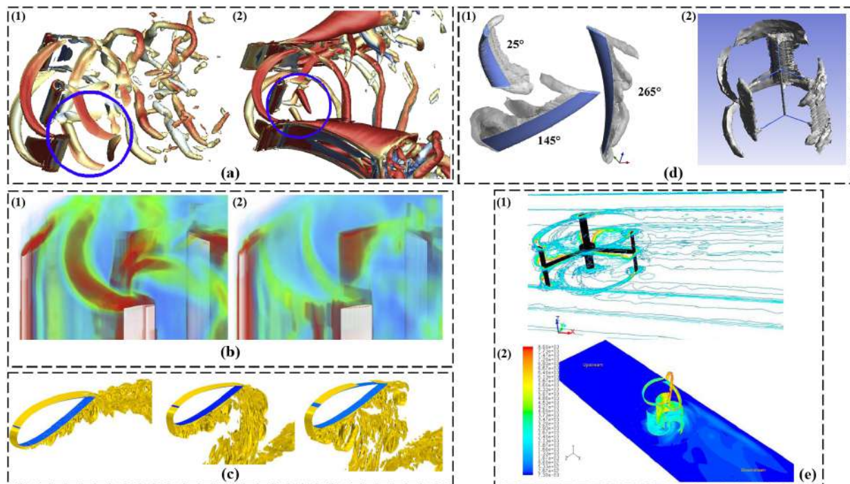
Figure 20. (a) Wake of the Darrieus VAWT for an open turbine (1) and a cycloidal surface diffuser wind lens (2). (reproduced with permission from Dessoky, Energy , published by ELSEVIER, 2019 [35]), (b) comparison of tip vortex generated by the J-shaped blades (1) and conventional blades (2) at a same azimuth position (reproduced with permission from Zamani, Energy , published by ELSEVIER, 2016 [54]), (c) Q-criterion (isosurface 300 \text{ s}^{-2} ) for three configurations of the rotating Darrieus modeled by LES (reproduced with permission from Patil, Energy , published by ELSEVIER, 2018 [20]), (d) (1) contour of the vorticity magnitude (3-PB configuration): iso surface of 65 \text{ s}^{-1} at a wind speed of 7 \text{ m/s} , rotational speed of 120 \text{ rpm} , and azimuth angle of 25 \text{ deg} . (2) Vortex shedding visualization for near turbine at vorticity of 16 \text{ ms}^{-1} at inflow 1 \text{ m/s} (reproduced with permission from Karimian, Energy , published by ELSEVIER, 2020, and from Tunio, Renewable Energy , published by ELSEVIER, 2020 [18,82]), and (e) (1) SB-VAWT: Contours of vorticity on 2D planes while turbine is mounted at 7.5c and operating at Tip Speed Ratio (TSR) of 3.0 . (2) Vorticity distribution (in per s) on horizontal cut planes at y = 0.05 \text{ m} (reproduced with permission from Siddiqui, Renewable Energy , published by ELSEVIER, 2021, and from Ghosh, Journal of the Energy Institute , published by ELSEVIER, 2015 [17,73]).
