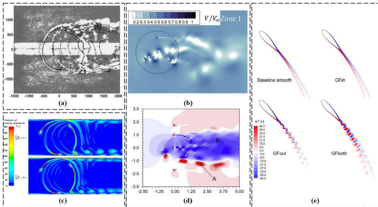
Figure 18. (a) Shed vortex centers path for a three-bladed Darrieus. Comparison of experimental visualization (Strickland JH et al.) and FEVDTM prediction (reproduced with permission from Ponta, Renewable energy , published by ELSEVIER, 2001 [13]), (b) dimensionless velocity magnitude around the blades for Zone 1 (reproduced with permission from Celik, Journal of Wind Engineering and Industrial Aerodynamics , published by ELSEVIER, 2020 [25]), (c) contours of vorticity magnitude (reproduced with permission from Marco, Procedia Computer Science , published by ELSEVIER, 2013 [45]), (d) normalized velocity in the wake at TSR = 1.4 (computed velocity field) (A: corresponds to powerful vortices that detach upwind from the blades and are subsequently carried downstream by the flow. The strength of these vortices might have been overestimated in CFD simulations compared to experimental observations. B: corresponds to an excessive reduction in velocity within the wake of the tower, a phenomenon that is not observed in experimental results) (reproduced with permission from Bianchini, Energy Conversion and Management , published by ELSEVIER, 2017 [56]) and (e) dimensionless vorticity contours ( TSR = 6.0 , vs. = 312 degree, h_{GF} = 2\% ) (reproduced with permission from Bianchini, Energy conversion and management , published by ELSEVIER, 2019 [1]).
