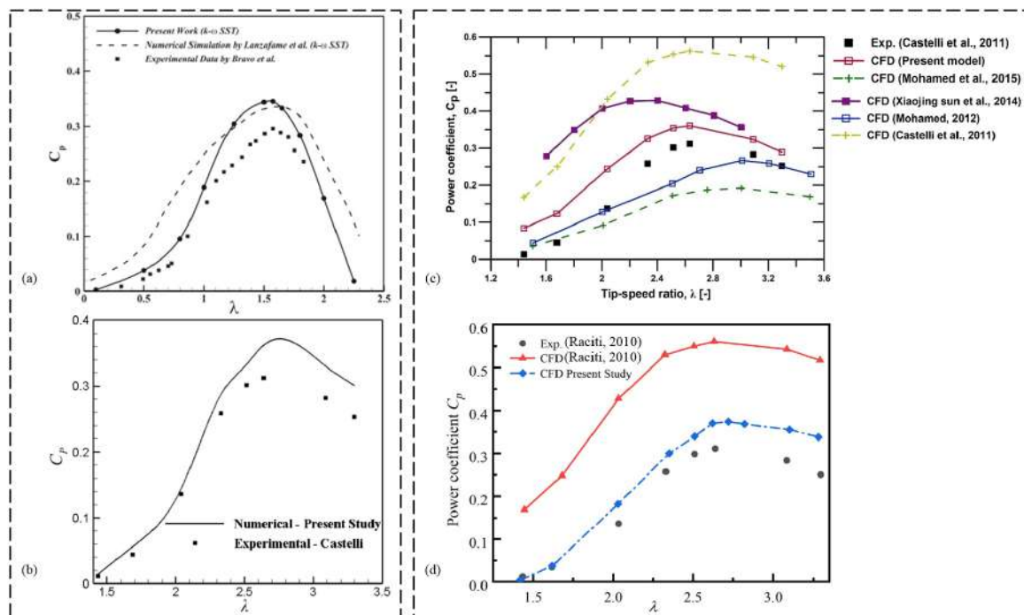
Figure 16. (a) Comparison of numerical results and experimental data by Bravo et al. (reproduced with permission from Zamani, Renewable Energy , published by ELSEVIER, 2016 [53]), (b) comparison of numerical and experimental results (reproduced with permission from Sobhani, Energy , published by ELSEVIER, 2017 [58]), (c) validation of present computational model, compared to experimental data for open Darrieus turbine and other computational results for Darrieus [40,46,47,65,78] (reproduced with permission from Hashem, Energy , published by ELSEVIER, 2018 [40]), and (d) power coefficient comparison between computation results and experiment values [79] (reproduced with permission from Ni, Energy , published by ELSEVIER, 2021 [71]).
