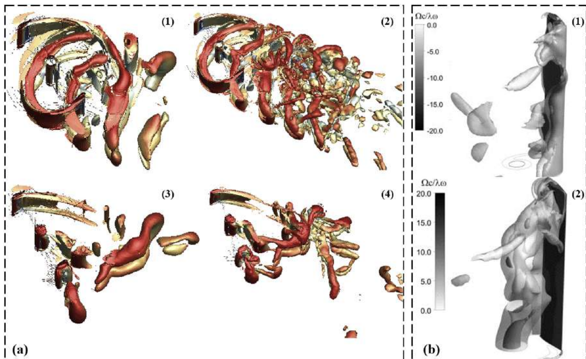
Figure 21. (a) (1) Wake of the Darrieus VAWT with different turbulence resolving approaches and speed ratio: URANS-JST/ \lambda = 2.75 , (2) DDES-WENO/ \lambda = 2.75 , (3) URANS-JST/ \lambda = 0.75 and (4) DDES-WENO/ \lambda = 0.75 (reproduced with permission from Dessoky, Renewable Energy , published by ELSEVIER, 2019 [36]), and (b) 3D view of the dimensional vorticity ( \frac{\Omega c}{\lambda V} ) for \theta = 120 deg; (1) positive vorticity; (2) negative vorticity (reproduced with permission from Rossetti, Renewable Energy , published by ELSEVIER, 2013 [31]).
