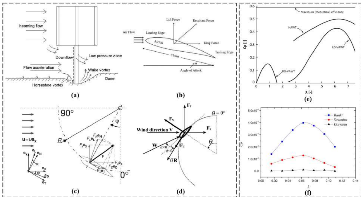
Figure 5. (a) Schematic diagram of scour topography around Darrieus-type tidal current turbine (reproduced with permission from Wei Haur Lam, Energy Conversion and Management , published by ELSEVIER, 2018 [6]), (b) forces acting on an airfoil (reproduced with permission from Ozkan, Renewable Energy , published by ELSEVIER, 2020 [7]), (c) schematic representation of the conventions used for Darrieus in the current study (reproduced with permission from Daroczy, Energy , published by ELSEVIER, 2015 [8]), (d) rotating directions and forces as a function of azimuthal angle (reproduced with permission from Nguyen, Journal of Wind Engineering and Industrial Aerodynamics ; published by ELSEVIER, 2020 [9]), (e) typical power coefficients for HAWT, DD-VAWT and LD-VAWT and the Betz limit C_p = 0.59 (reproduced with permission from Trivellato, Renewable and Sustainable Energy Reviews , published by ELSEVIER, 2015 [10]), and (f) power coefficients for different Darrieus wind turbines (reproduced with permission from Mao, Renewable Energy , published by ELSEVIER, 2020 [11]).
