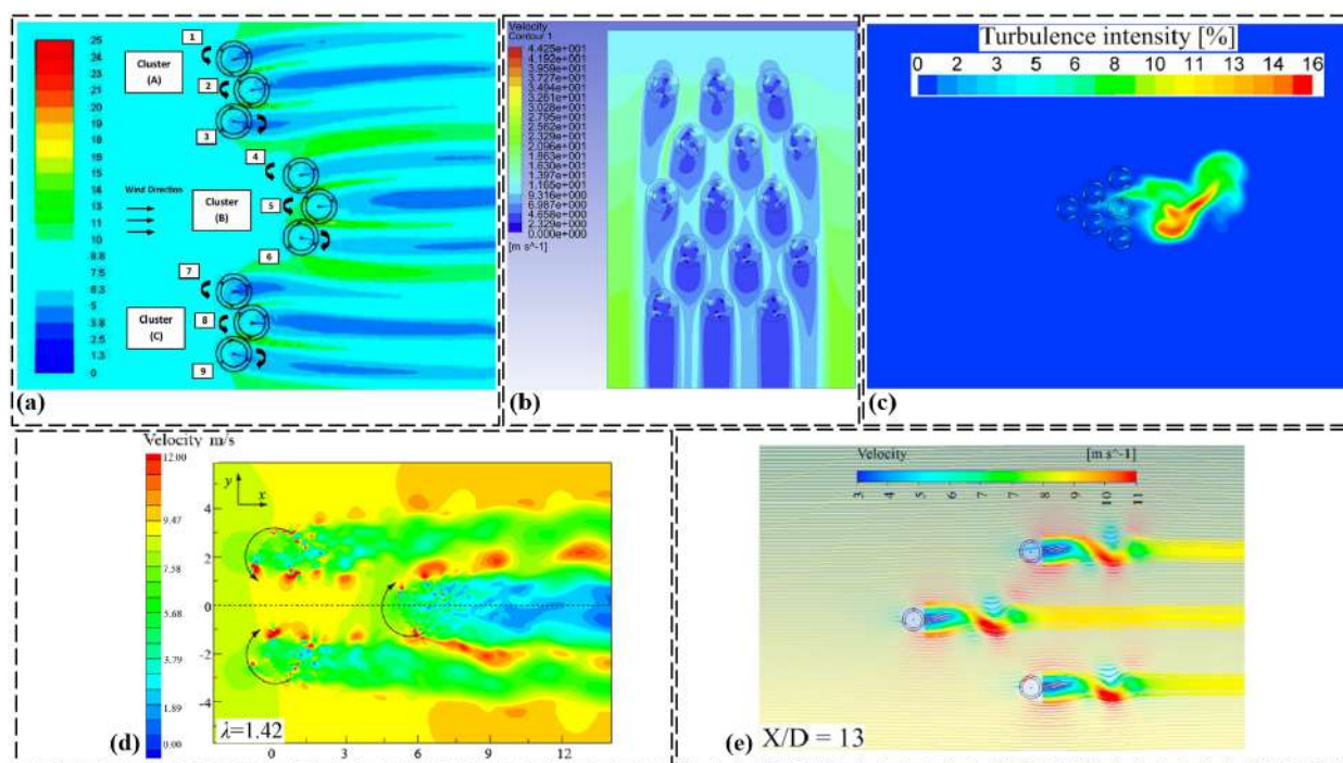
Figure 19. (a) Velocity contours around a nine savonius wind turbine farm (reproduced with permission from Shaheen, Sustainable Energy Technologies and Assessments , published by ELSEVIER, 2017 [57]), (b) velocity contour map for a 3 \times 5 farm with spacing x = 5 , y = 10 (reproduced with permission from Barnes, Renewable energy , published by ELSEVIER, 2019 [62]), (c) turbulence intensity of the six turbine cluster at X/D = 1.5 and \lambda = 3.3 (reproduced with permission from Shaaban, Renewable Energy , published by ELSEVIER, 2018 [59]), (d) the wake velocity contours at the tip speed ratio of 1.42 (reproduced with permission from Ni, Energy , published by ELSEVIER, 2021 [71]), and (e) pathlines for the three equilateral turbine cluster at X/D = 13 (reproduced with permission from Shaaban, Renewable Energy , published by ELSEVIER, 2018 [59]).
