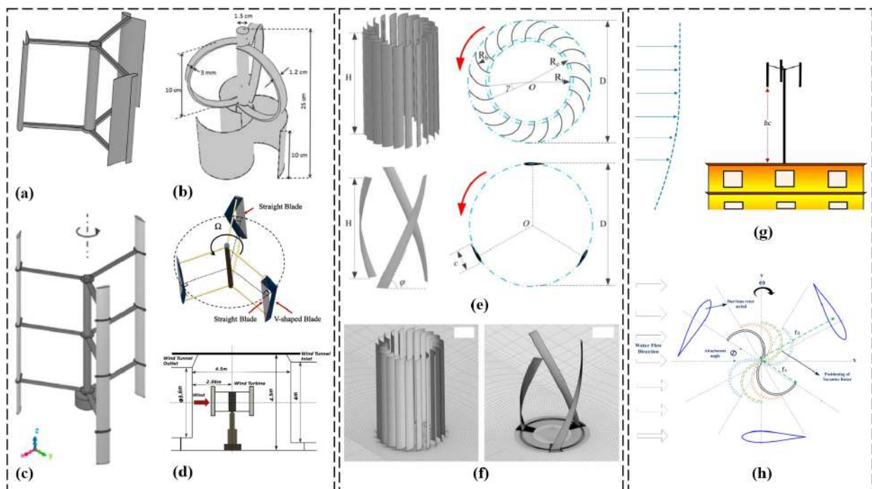
Figure 14. (a) The schematic representation of a Darrieus VAWT with the J-shaped section (reproduced with permission from Zamani, Energy , published by ELSEVIER, 2016 [54]), (b) combined three-bladed Darrieus and three-bladed bucket Savonius (reproduced with permission from Ghosh, Journal of the Energy Institute , published by ELSEVIER, 2015 [17]), (c) geometric details of wind turbine model for CFD simulation (perspective view) (reproduced with permission from Ali, Energy Conversion and Management , published by ELSEVIER, 2018 [60]), (d) the sketch map of the VAWT with V-shaped blade (transformation of the three-dimensional model)/schematic sketch of experimental apparatus (reproduced with permission from Dessoky, Energy , published by ELSEVIER, 2019 [35]), (e) three VAWTs in the simulation: Banki turbine (Top Configuration); Darrieus (Bottom Configuration) (reproduced with permission from Tian, Renewable Energy , published by ELSEVIER, 2020 [11]), (f) details of the computation mesh: grids around the Banki turbine; grids around the Darrieus (reproduced with permission from Tian, Renewable Energy , published by ELSEVIER, 2020 [11]), (g) SB-VAWT: the schematic of turbine placed on a rooftop illustrating variations in height; five levels of height are considered, i.e., 1.0c (Case i), 2.5c (Case ii), 4.0c (Case iii), 7.5c (Case iv), and 10.0c (Case v) (reproduced with permission from Siddiqui, Renewable Energy , published by ELSEVIER, 2021 [73]), and (h) schematic of a hybrid Darrieus (reproduced with permission from Saini, Ocean Engineering , published by ELSEVIER, 2020 [15]).
