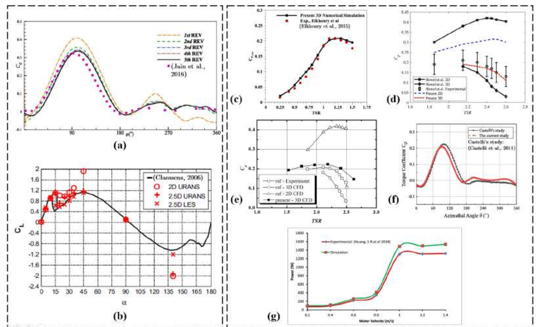
Figure 17. (a) Comparison of the torque coefficient in the first five revolutions with the test result, \lambda = 2.29 [80] (reproduced with permission from Xu, Energy Conversion and Management , published by ELSEVIER, 2020 [63]), (b) lift coefficient of NACA0018 airfoil for Re = 300,000 [77] (reproduced with permission from Li, Renewable energy , published by ELSEVIER, 2013 [14]), (c) comparison between averages of the total power coefficient of experimental data by Elkhoury et al. [81] and 3D results presented in [18] (reproduced with permission from Karimian, Energy , published by ELSEVIER, 2020 [18]), (d) SB-VAWT: results are benchmarked with Howel et al. [73] experimental and numerical results (reproduced with permission from Siddiqui, Renewable Energy , published by ELSEVIER, 2021 [73]). Experimental results have been reported at a wind speed of 5.07 m/s. The numerical results are within the \pm 20\% error range and more realistic than Howel et al. results at higher TSRs (reproduced with permission from Siddiqui, Renewable Energy , published by ELSEVIER, 2021 [73]), (e) power coefficient comparison between the computational and experimental results by Robert et al. (reproduced with permission from Joo, Energy , published by ELSEVIER, 2015 [34]), (f) comparison of the dynamic torque coefficient at tip speed ratio \lambda = 3.1 (Castelli et al. [65]) (reproduced with permission from Su, Applied Energy , published by ELSEVIER, 2020 [38]), and (g) computational model validation with published experimental data at different values of TSR (reproduced with permission from Tunio, Renewable Energy , published by ELSEVIER, 2020 [82]).
