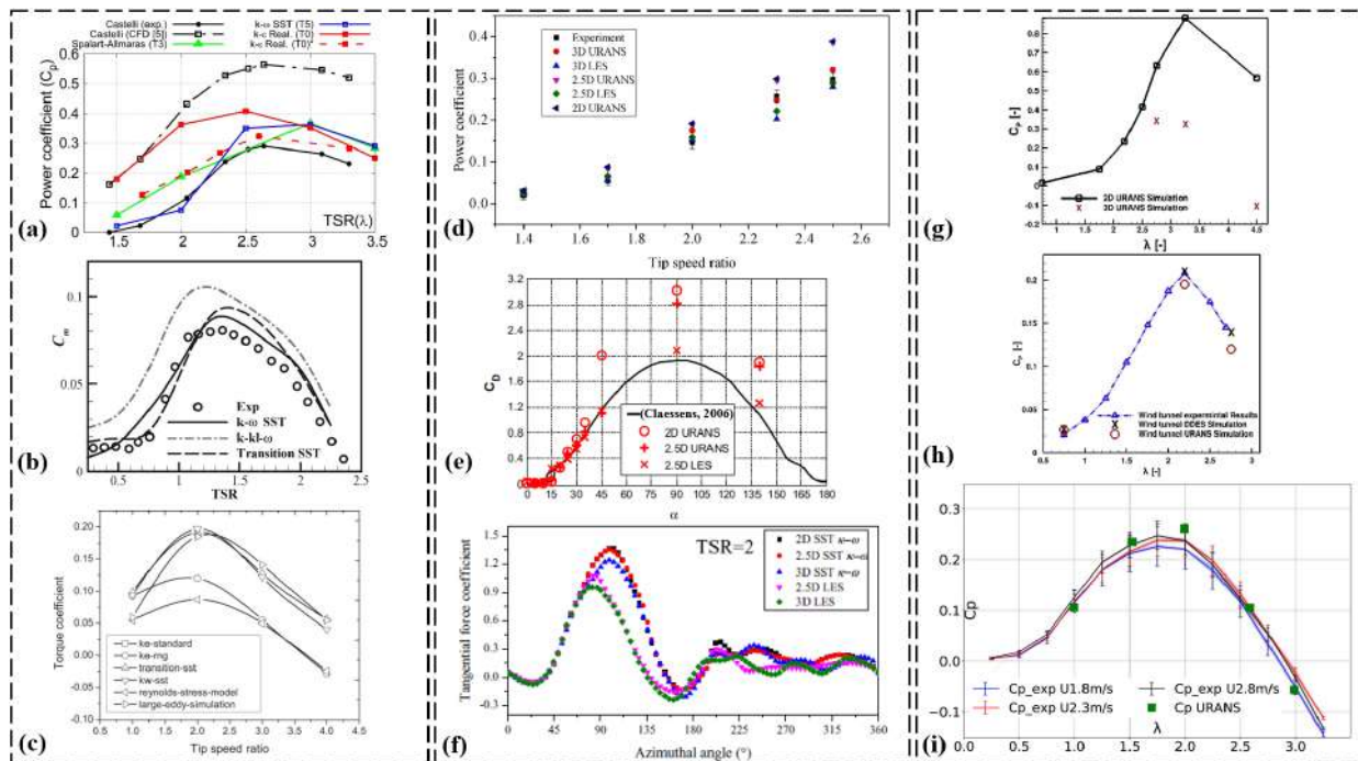
Figure 15. (a) Experimental validation based on Castelli et al. [65](exp) (reproduced with permission from Daroczy, Energy , published by ELSEVIER, 2015 [8]), (b) the numerical results comparison with the experimental data of Takao et al., using various turbulence models (reproduced with permission from Arab, Renewable Energy , published by ELSEVIER, 2017 [24]), (c) effect of different turbulence models on the simulation results (reproduced with permission from Chen, Energy , published by ELSEVIER, 2015 [50]), (d) comparison of experimental and simulated C_p at different TSRs (reproduced with permission from He, Renewable Energy , published by ELSEVIER, 2020 [30]), (e) lift and drag coefficients of NACA0018 airfoil for Re = 300,000 [77] (reproduced with permission from Li, Renewable energy , published by ELSEVIER, 2013 [14]), (f) tangential force coefficients of a single blade against the azimuthal angle for various CFD schemes (TSR = 2) (reproduced with permission from He, Renewable Energy , published by ELSEVIER, 2020 [30]), (g) comparison of the power coefficient ( C_p ) curves between 2D and 3D URANS CFD simulations (reproduced with permission from Dessoky, Energy , published by ELSEVIER, 2019 [35]), (h) comparison of power coefficient ( C_p ) curve of Darrieus VAWT model (reproduced with permission from Dessoky, Energy , published by ELSEVIER, 2019 [35]), and (i) comparison of the experimental and URANS blade-resolved simulation C_p curves (reproduced with permission from Clary, Ocean Engineering , published by ELSEVIER, 2020 [37]).
