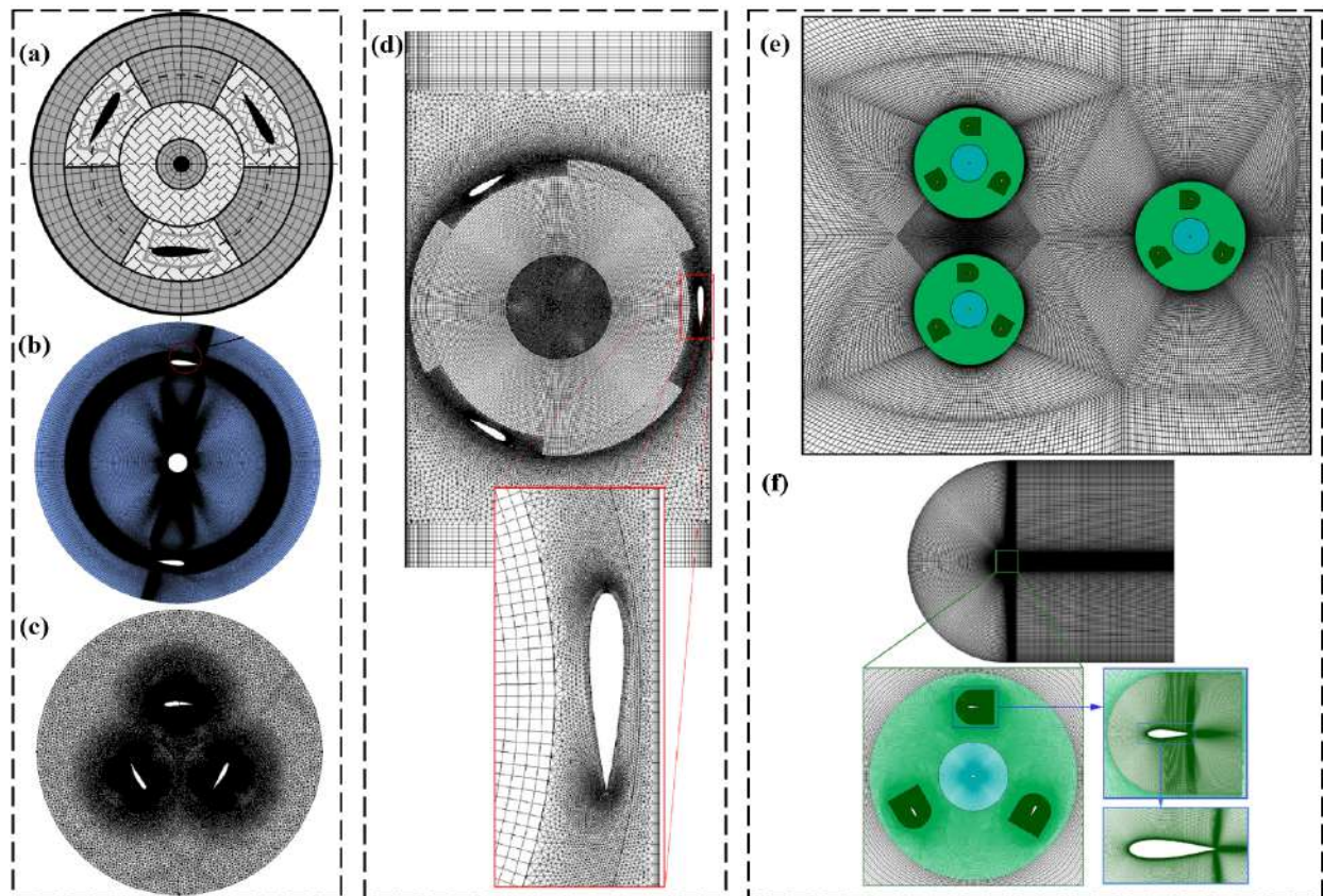
Figure 8. (a) Rotating domain of the mesh (reproduced with permission from Daroczy, Energy , published by ELSEVIER, 2015 [8]), (b) wind-lens (reproduced with permission from Dessoky, Energy , published by ELSEVIER, 2019 [35]), (c) the rotating zone (reproduced with permission from Arab, Renewable Energy , published by ELSEVIER, 2017 [24]), (d) details of the mesh in the zone swept by the Darrieus (reproduced with permission from Torresi, Procedia Computer Science , published by ELSEVIER, 2013 [45]), (e) mesh distribution of VAWTs in array configurations (reproduced with permission from Ni, Energy , published by ELSEVIER, 2021 [71]), and (f) computational mesh distributions (reproduced with permission from Ni, Energy , published by ELSEVIER, 2021 [71]).
