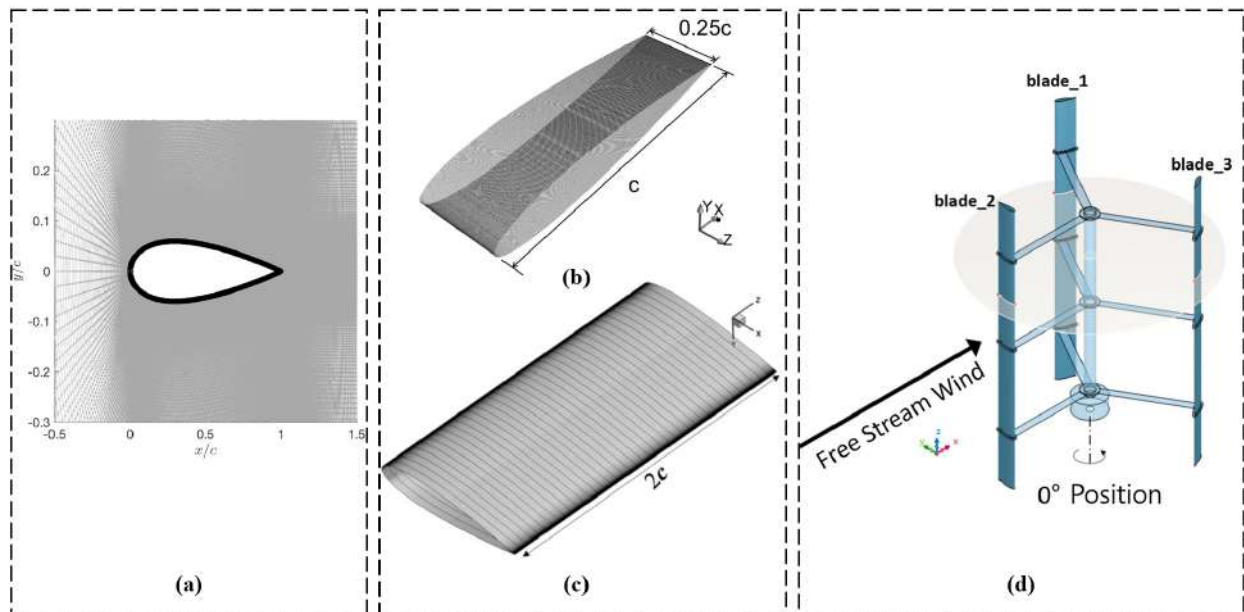
Figure 6. (a) 2D modeling: close-up view of the mesh around the airfoil (reproduced with permission from Atlaschian, Renewable Energy , published by ELSEVIER, 2021 [68]), (b) 2.5D modeling: computational grid of the turbine for the SAS simulation with a total of 19,753,402 quadrilateral cells (reproduced with permission from Reazeiha, Energy Conversion and Management , published by ELSEVIER, 2019 [29]), (c) 2.5D modeling: mesh distribution for single static NACA0018 airfoil (reproduced with permission from Zhu, Renewable Energy , published by ELSEVIER, 2013 [14]), (d) 3D modeling: definition of blade numbers and 0 degree azimuthal position (reproduced with permission from Jang, Energy Conversion and Management , published by ELSEVIER, 2018 [60]).
