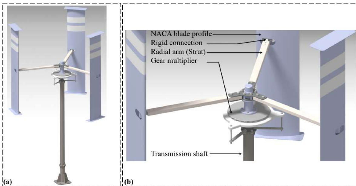
Figure 2. (a) Prototype of Darrieus wind turbine. (b) Mechanical transmission system of Darrieus.
