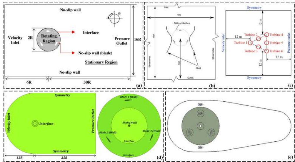
Figure 11. (a) Computational domain and boundary conditions (reproduced with permission from Arab, Renewable Energy , published by ELSEVIER, 2017 [24]), (b) schematic of the computational domain in case of ducted turbine (reproduced with permission from Malipeddi, Renewable Energy , published by ELSEVIER, 2012 [44]), (c) computational domain of a 6 turbine cluster (reproduced with permission from Shaaban, Renewable Energy , published by ELSEVIER, 2018 [59]), (d) principal dimensions and boundary conditions of computational domain (reproduced with permission from Zamani, Energy , published by ELSEVIER, 2016 [54]), and (e) mesh refinement in the wake (reproduced with permission from Bianchini, Energy Conversion and Management , published by ELSEVIER, 2017 [56]).
