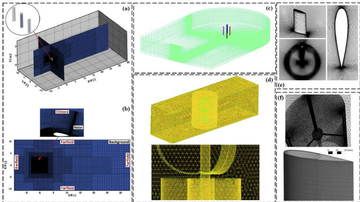
Figure 10. (a) Sectional 3D computational mesh used in the simulations (reproduced with permission from Dessoky, Energy , published by ELSEVIER, 2019 [35]), (b) computational mesh used in the simulations: background (reproduced with permission from Dessoky, Energy , published by ELSEVIER, 2019 [35]), (c) mesh structure of the 3D computational domain (reproduced with permission from Zamani, Energy , published by ELSEVIER, 2016 [54]), (d) computational mesh around combined Darrieus and the front view of the mesh very near to the blades (reproduced with permission from Ghosh, Journal of the Energy Institute , published by ELSEVIER, 2015 [17]), (e) some details of the computational mesh (reproduced with permission from Balduzzi, Energy , published by ELSEVIER, 2017 [16]), and (f) SB-VAWT: generated mesh for the three-dimensional (3D) models of turbine using Sliding Mesh Interface (SMI) (zoomed Darrieus view) and 3D mesh on blade tip (reproduced with permission from Siddiqui, Renewable Energy , published by ELSEVIER, 2021 and Rossetti, Renewable Energy , published by ELSEVIER, 2013 [31,73]).
