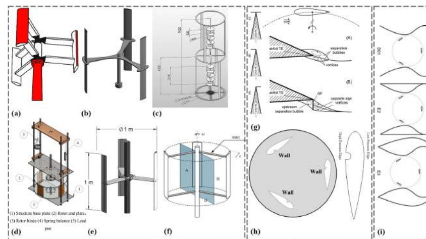
Figure 13. (a) Darrieus wind turbine (reproduced with permission from Hashem, Energy , published by ELSEVIER, 2018 [40]), (b) straight-bladed Darrieus schematic (reproduced with permission from Asr, Energy , published by ELSEVIER, 2016 [41]), (c) the final assembly (dimensions in mm) (reproduced with permission from Hosseini, Energy conversion and management , published by ELSEVIER, 2019 [72]), (d) schematic representation of the experimental set up (reproduced with permission from Patel, International journal of marine energy , published by ELSEVIER, 2017 [61]), (e) CAD of the assessed Darrieus turbine (reproduced with permission from Bianchini, Energy Conversion and Management , published by ELSEVIER, 2017 [56]), (f) schematic view of the architecture of the analyzed Darrieus turbines (reproduced with permission from Bianchini, Energy conversion and management , published by ELSEVIER, 2015 [19]), (g) different compared GF configurations: (left (A) GF in configuration; (B) GF out configuration; (C) GF both configuration). (right (A) flow field around smooth airfoil; (B) hypothesized flow field around an airfoil with a Gurney flap (reproduced with permission from Bianchini, Energy conversion and management , published by ELSEVIER, 2019 [1])), (h) computational domain and boundary conditions (reproduced with permission from Sobhani, Energy , published by ELSEVIER, 2017 [58]), and (i) the different external shapes for which the simulations were performed (reproduced with permission from Malipeddi, Renewable Energy , published by ELSEVIER, 2012 [44]).
