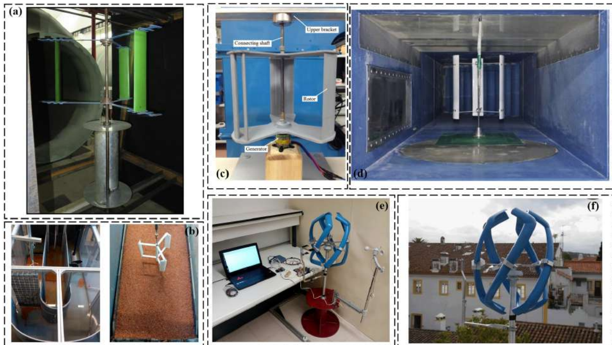
Figure 22. (a) Photograph showing the two hybrid turbines used in the experiments (reproduced with permission from Jacob, Renewable Energy , published by ELSEVIER, 2019 [67]), (b) experimental setup of model and instrumentation (reproduced with permission from Sun, Energy Conversion and Management , published by ELSEVIER, 2018 [6]), (c) connection of the Darrieus-generator and support system (reproduced with permission from Scungio, Energy Conversion and Management , published by ELSEVIER, 2016 [83]), (d) solid plate and Darrieus turbine installed in three different wind tunnels (wind tunnel-C, blockage ratio: 24.70%) (reproduced with permission from Jeong, Journal of Wind Engineering and Industrial Aerodynamics , published by ELSEVIER, 2018 [84]), (e) prototype and sensors (reproduced with permission from Pereira, Energy , published by ELSEVIER, 2018 [85]), and (f) new Darrieus VAWT design prototype (reproduced with permission from Batista, Renewable and Sustainable Energy Reviews , published by ELSEVIER, 2015 [86]).
