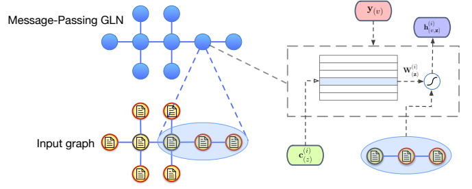
Fig. 1: A graphical layout of the proposed Message-Passing GLN, with an expanded view of the GLN neuron.
