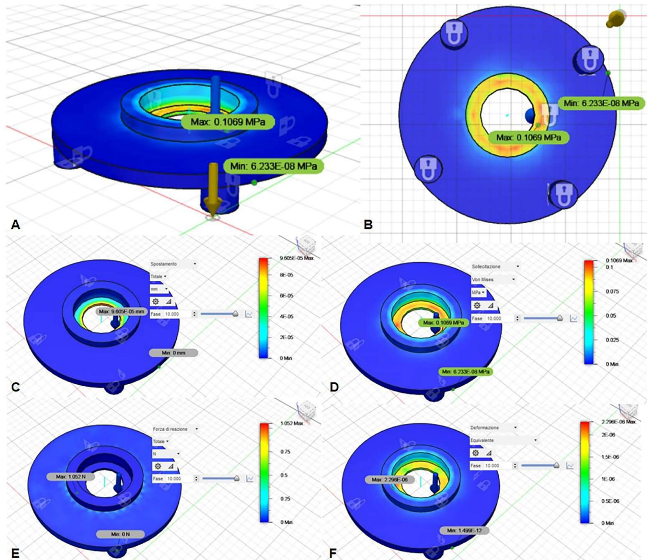
Figure 2. Mechanical simulation of the material used for the support, using Autodesk Fusion 360 (Autodesk, Inc., San Rafael, CA, USA): (A) lateral view; (B) bottom view; (C) shift assessment; (D) stress assessment; (E) reaction force assessment; (F) strain assessment.
