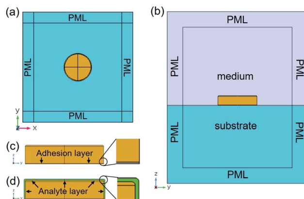
Fig. 1 Geometry of the FEM model. (a) Top view ( \widehat{xy} plane) and (b) side view ( \widehat{yz} plane) of the simulation cell. The lower part of the model (aqua) has the silica refractive index n_{\text{sub}} = 1.45 , while the upper part (light purple) has the refractive index of air ( n_{\text{med}} = 1 ) or of the simulated bulk environment. (c and d) Side views of a nanodisk in which it is highlighted the presence of an adhesion layer ( t_{\text{adh}} = 2 nm) of Cr below the nanodisk (c), and a t_{\text{a}} -thick layer of analyte (green) all around the nanodisk (d).
