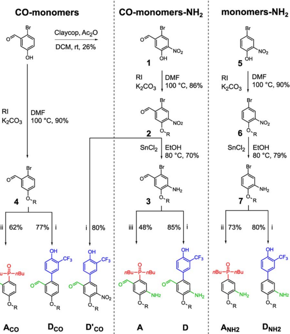
Scheme 1 Synthesis of acceptor and donor monomers (R = 2-ethylhexyl). (i) \text{Pd}_2(\text{dba})_3 , KF, \text{HP}(\text{tBu})_3\text{BF}_4 , 4-pinacolborane-2-(trifluoromethyl)phenol, THF/ \text{H}_2\text{O} ; (ii) \text{Pd}_2(\text{dba})_3 , XantPhos, TEA, \text{PHOBU}_2 , dioxane; (iii) CuI, \text{PHOBU}_2 , \text{Na}_2\text{CO}_3 , toluene.
