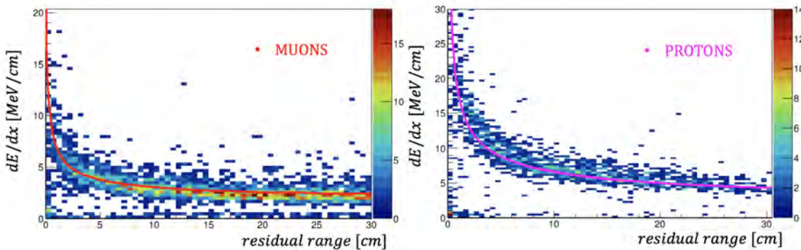
Figure 2: Deposited energy along the trajectory for muon and proton candidates. The theoretical stopping power for each particle is also shown.
