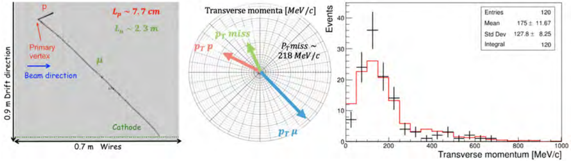
Figure 3: Left: \nu_\mu CC quasi-elastic event collected with BNB. Middle: transverse momentum reconstruction of the previous event. Right: neutrino transverse momenta distribution for all well reconstructed events in comparison to MC expectations.
