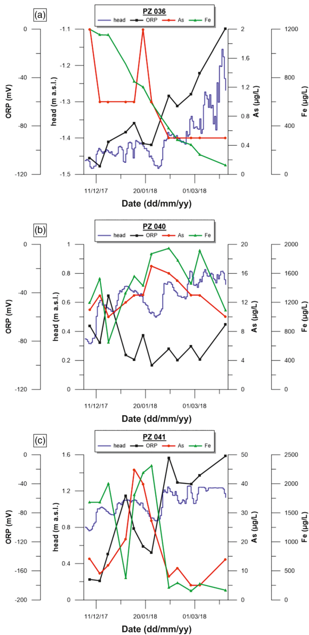
Figure 3. Time series of measured variations of groundwater head, oxidizing-reduction potential (ORP), and arsenic (As) and iron (Fe) concentrations for the three piezometers PZP036 (a), PZP040 (b), and PZP041 (c), with weekly geochemical monitoring and continuous groundwater head level logging.
