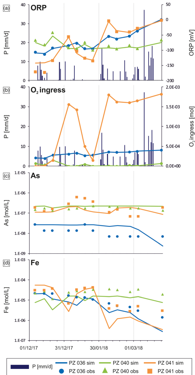
Figure 6. Comparison between observed (symbols) and simulated (lines) variables for PZP036, PZP040, and PZP041. Panel (a) shows the comparison for ORP. Panel (b) reproduces the shape of the rate-limiting function that enables reproducing the observed ORP at the three piezometers. The observed daily rainfall depths ( P ) is reported in both Panels (a) and (b). Panel (c) shows the comparison for As, and Panel (d) for Fe.
