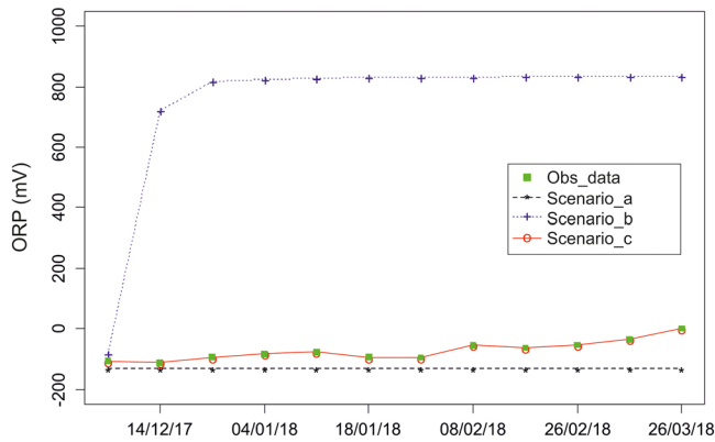
Figure 5. Comparison between measured ORP at PZP036 and simulated using PHREEQC models embedding the three different scenarios (a–c). Each scenario describes a specific modality of oxidants transfer from the surface to the aquifer.
