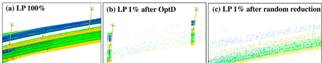
Figure 4. Effect of the data reduction on an area containing LPs: (a) original view, (b) point cloud after OptD method, (c) point cloud after random reduction.
