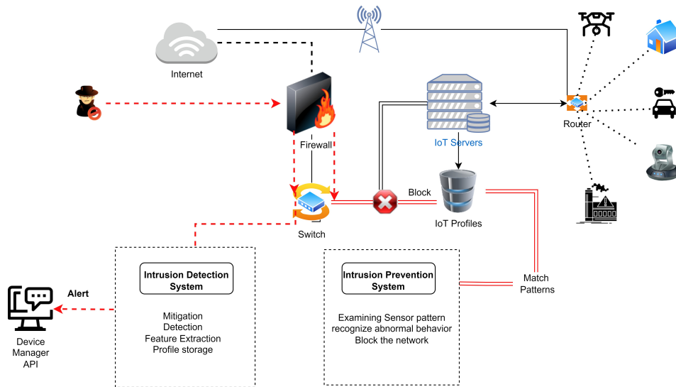
FIGURE 1: IDPS Architecture
