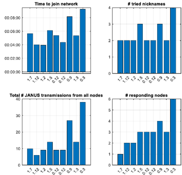
Fig. 12. Time to join the network, number of tried nicknames, total number of JANUS transmissions from all nodes and number of responding nodes, for a sequence of nodes using the first-contact mechanism during harbour tests in Motala (HAT2, 2021). The nodes are plotted in the order that they joined, from left to right.
