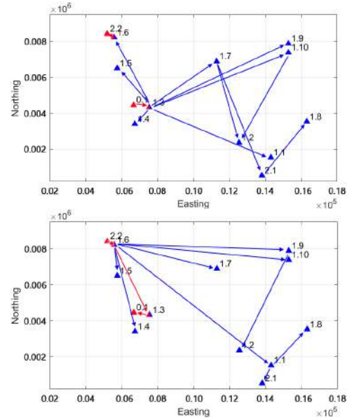
Fig. 9. Simulations of multi-topology routing, i.e., communication through LF (blue) and HF (red) frequency bands. Top: Request from gateway buoy 0.1 to AUV 2.2. Bottom: Reply from 2.2 to 0.1.
