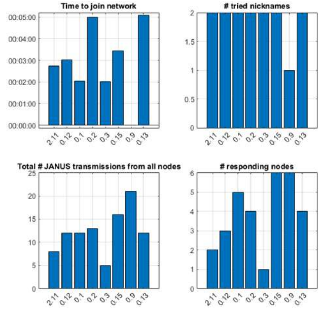
Fig. 16. Time to join the network, number of tried nicknames, total number of JANUS transmissions from all nodes and number of responding nodes, for a sequence of nodes using the first-contact mechanism during harbour tests in Horten (HAT3, 2022). The nodes are plotted in the order that they joined, from left to right.
