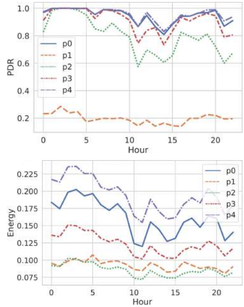
Fig. 10. Simulations of AMC PDR and energy performance: p1-p4 are fixed data rates (with p4 most robust), while p0 uses dynamic switching. [12]
