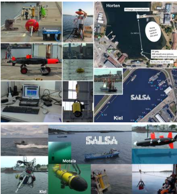
Fig. 11. Impression of the SALSA harbour tests in 2020 (Kiel/Horten; top) and 2021 (Motala/Kiel; bottom).
