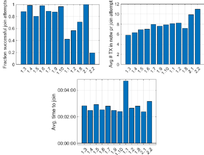
Fig. 8. Simulated first-contact protocol performance for each joining node, averaged over different time offsets in the Look-Up Tables (LUTs). [14]
