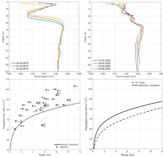
Fig. 3. Sound-speed profiles (top) as measured in the Oslofjord in April/May 2019 (left) [10] and 2022 (right), and propagation loss (bottom) in the 4-8 kHz band as measured in the Oslofjord in April/May 2019 (left) [10]. The indices of the propagation-loss measurements indicate the links between the (NILUS) bottom nodes (link N5→N6 is denoted by 56, etc.). For comparison, modelled propagation loss is also shown (bottom-right), using the (depth-independent) Thiele formula [11] of the network simulator (blue dashed line) and spherical spreading + absorption (solid black line) at f_c = 6 kHz.
