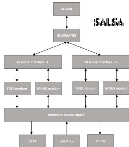
Fig. 5. SALSA software-defined modem architecture indicating the separate processes for the application layer (GUWAL), the network layer (GUWMANET), the low-frequency (LF) and high-frequency (HF) bands, and the FRSS-SALSA and JANUS modulations.
