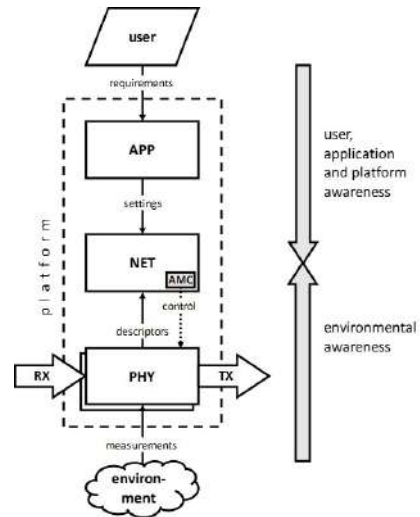
Fig. 4. SALSA network-communications protocol stack, indicating external influences (user, environment) and directions of information flow, the capabilities at each layer and their interrelations, and the ‘NET-centric’ Adaptive Modem Configuration (AMC) module.
