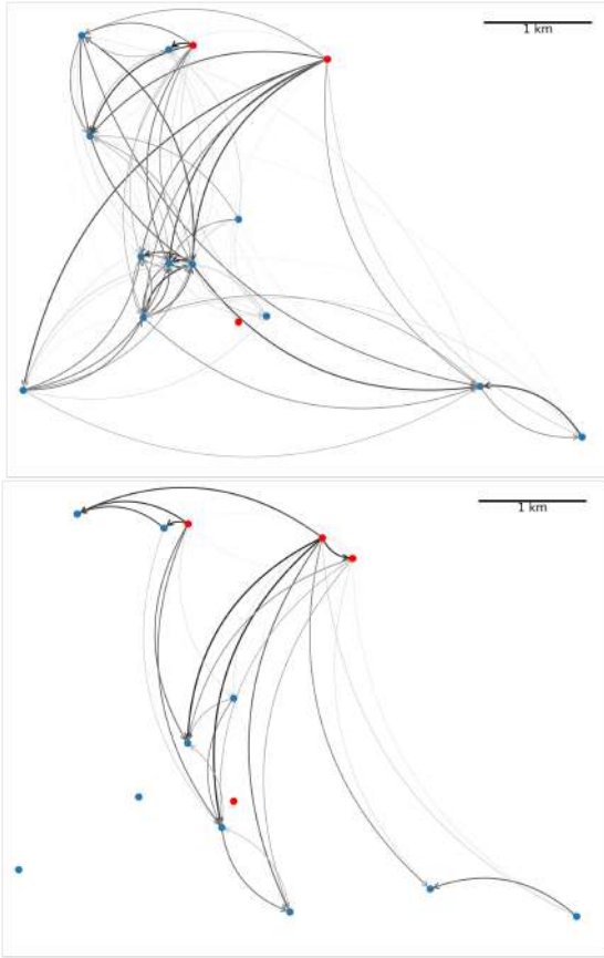
Fig. 15. Physical-layer connectivity maps for the LF band (top) and the HF band (bottom) in the Oslofjord on 3 May, 09:52-16:00 UTC (arrows pointing counter-clockwise, grayscale indicating PDR). Both panels show many asymmetric links and better LF connectivity than HF connectivity. Some long-range connections were with mobile nodes (red dots) plotted at their nominal positions.
