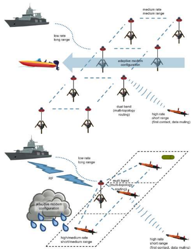
Fig. 1. A schematic ISR network scenario (top) for detecting mobile targets, consisting of mainly fixed barrier nodes and mobile reconnaissance node(s), and a schematic MCM/REA network scenario (bottom) for detecting stationary targets, consisting of mainly mobile survey nodes and fixed gateway node(s). Both networks may be operated from a mothership over the horizon. From an underwater-communications perspective, these can be considered as two “extreme” scenarios. Practical scenarios are likely to be more mixed static/mobile (heterogeneous network).
