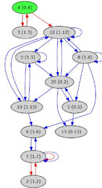
Fig. 17. Network connectivity analysis showing how nodes communicated with each other via LF/HF relay nodes in the Oslofjord (2022). Blue arrows indicate LF communication and red arrows indicate HF communication. The graph shows multi-topology routing of a broadcast packet. LF-only nodes are 0.2, 1.5 and 1.6; HF-only nodes are 0.4, 1.2 and 1.3; LF+HF nodes are 0.1, 0.13, 1.7, 1.8, 1.12 and 1.15.
