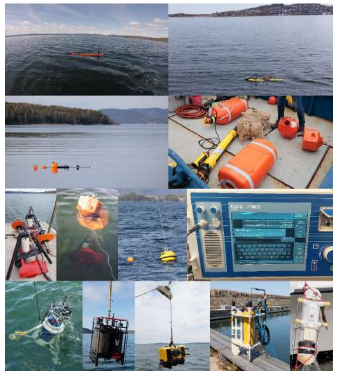
Fig. 14. Overview of network nodes deployed during the demonstration. Top-down/left-right: OceanScan LAUV (TNO), L3Harris Iver3 (Patria), Sea-Cat (ATLAS), cNode (Kongsberg), NILUS Mk2 (TNO), NILUS Mk2 with cNode (FFI), Gateway Buoy (FKIE), UT 3000 (ELAC), NEREUS Mk2 and Mk3 (WTD71), Bottom Lander (Develogic), Saab Sensor Node (Saab), and OnWeBSel (ATLAS). No ship nodes are shown.
