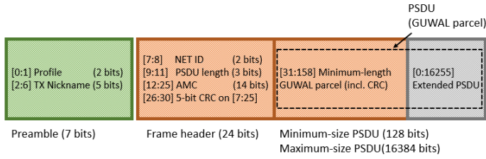
Fig. 6. Bit allocation for the coded preamble (green) and frame header with minimum-length packet size (orange) and with extended-length packet size (orange-gray). The “TX nickname” was included in the preamble to identify bad links.
