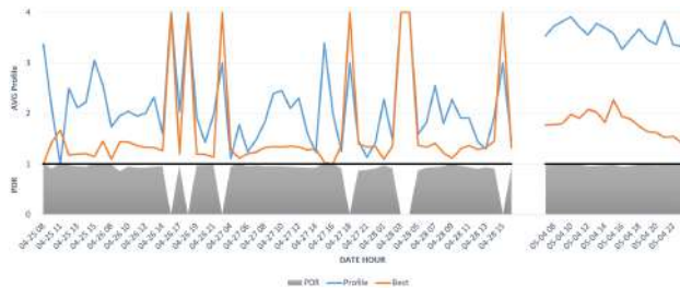
Fig. 18. AMC statistics (LF) for HAT3 (25-28 April 2022) and demo day (4 May 2022): Packet Delivery Ratio (PDR; gray), average selected FRSS profile (blue) and best profile (orange) for selected thresholds for the acoustic descriptors (as described in Sec. III-A).
