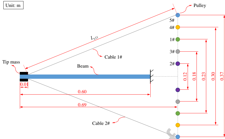
Fig. 11. Layout of five pulley locations for the flexible beam with two cables (dimensions in meters).
