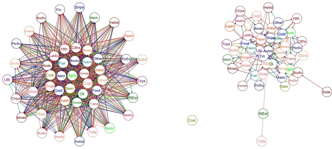
(a) Q_{10} Not Parametric
