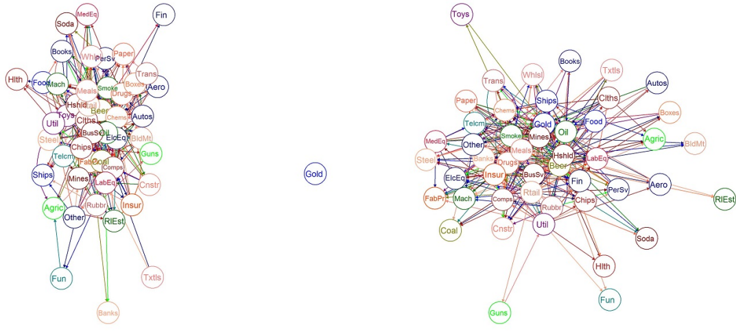
(c) Q_{90} Base Quantile
