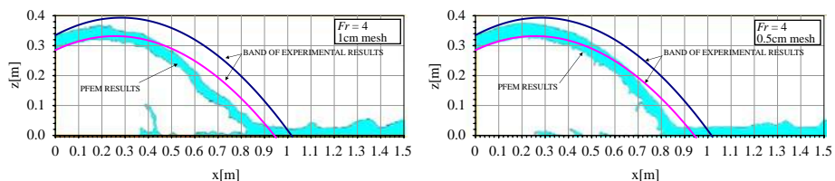
Figure 12. Flip bucket. Fr = 4 . Comparison between PFEM results and the band of experimental values for the jet trajectory
