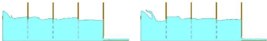
Figure 30. Sluice gate. Model 2. Simulation of the flow at different instances
