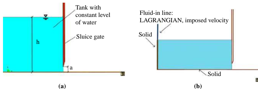
Figure 27. Sluice gate model. A detail
