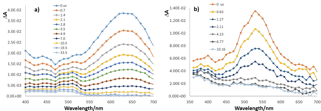
Figure 2. Time-resolved difference absorption spectra ( \Delta A ) flashing argon-purged acetonitrile solutions of 6e ( 1 \times 10^{-4} M) (a) and 5h ( 5 \times 10^{-4} M) (b), at 355 nm.
