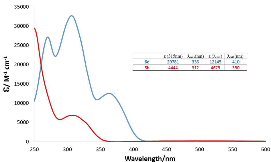
Figure 4. Absorbance comparison of 6e ( 10^{-4} M) and 5h ( 10^{-4} M) in acetonitrile: water = 3:2 solutions.
