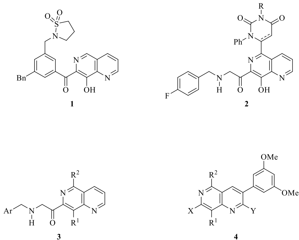
Chart 1. Structures of [1,6]naphthyridine derivatives 1-4.
