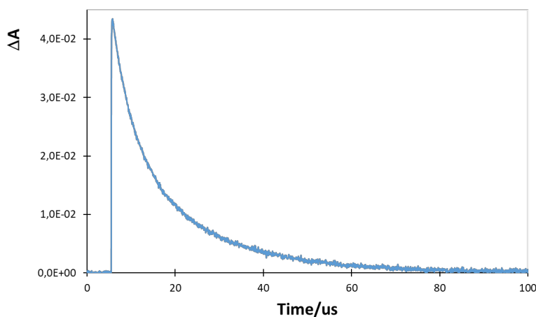
Figure 3. Triplet decay trace of 6e monitored at 630 nm in neat acetonitrile under argon saturated condition.
