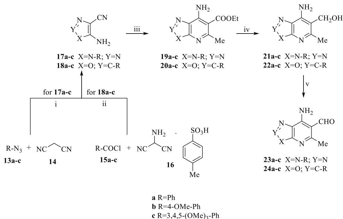
Scheme 1. Synthesis of key intermediates 23a-c , and 24a-c .
