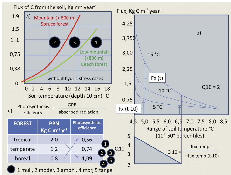
Fig. 32. Changes in carbon flux, soil temperature and photosynthesis efficiency. Examples from the Italian side of central Alps: beech forest model, in Rodeghiero (2003); spruce forest, in Rodeghiero and Cescatti (2005). a) Soil respiration (flux of C) increases exponentially with soil temperature. Humus systems are represented as black circles on the graph. Mull (black dot 1) was investigated only in a beech forest; Moder (2) was common in mountain spruce forests of the studied region (red line); Amphi (3) is well-known in the studied region at the altitudinal level of sub-mountain (600–800 m) to mountain (800–1300 m) forests. The three humus systems show a differential response in terms of carbon fluxes controlled by water content and soil temperature. b) The flux of C from the soil depends on soil temperature: the lower the temperature, the higher the Q10 (temperature coefficient), i.e. the rate of increase of C flux temperature is increased by 10 °C. Then, in a site with a low average annual temperature (example 5 °C in the graph), a sudden increase in temperature will rapidly generate a strong flux of carbon respired by the soil. This phenomenon can explain the presence of Mull at a relatively high altitude, even if the more common humus system at this altitude is Moder. Inversely, a low Q10 at lower elevation results in a slow response of soil microorganisms to changes in temperature and can explain the presence of undecomposed horizons like the OH of Amphi, instead of a usual Mull without OH horizon. c) Photosynthesis efficiency is higher in boreal
