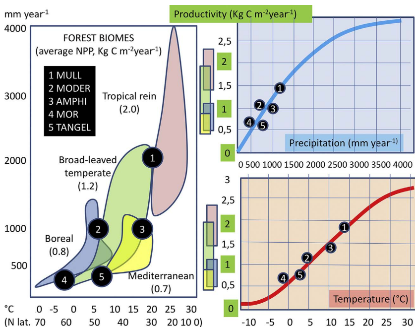
Fig. 24. Climate effects on production of carbon biomass. Carbon photosynthetic fixation (simplified from Lieth and Whittaker, 1975) has been related to average annual precipitation and air temperature (on the right). The main forest biomes have been placed on the left graph with the aim to show their “climatic amplitude” for the same parameters. Under the temperature x-axis, a corresponding north latitude degrees’ scale has been indicated. Between the two graphs, some coloured rectangles display the net primary productivity of each of these biomes. On the graphs, five black points indicate the hypothetical “attractor factor” for five main humus systems: Mull with highest precipitation-temperature values for a maximum primary production, Mor and Tangel with lowest values for these two climatic variables, Moder and Amphi with intermediate values.
