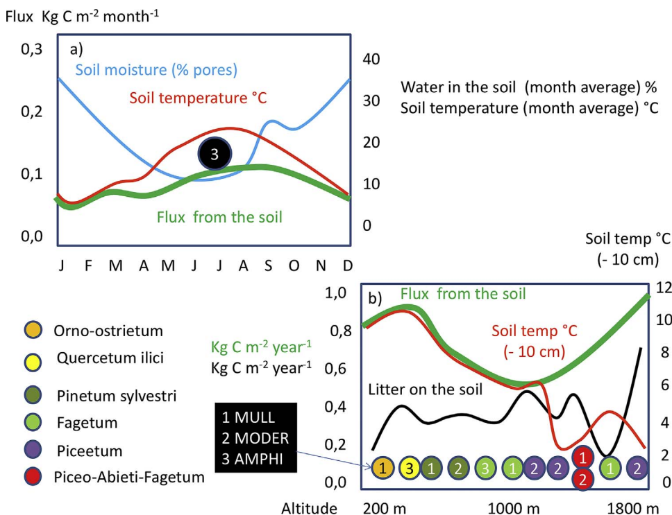
Fig. 33. Respiration in the soil along the year follows the curve of soil temperature if there is no water deficit (simplified from Rodeghiero, 2003: two years of data in continuum). a) Changes in C flux in relation to soil temperature and water content during one year (from J = January to D = December). Soil respiration (C flux) follows increases and decreases of temperature but is limited by water deficit during summer. This is the most probable explanation for the presence of an Amphi system (black circle). If this drier period of the year is long enough, soil respiration becomes arrested and organic horizons are formed in the upper part of the topsoil. b) Vertical axis: left, C flux from the soil, C content in annual fallen litter; right axis: soil temperature; horizontal axis: elevation. Little coloured circles correspond to vegetation and associated humus systems. Up to 1000 m elevation, soil C fluxes and temperatures change in parallel; from 1000 to 1800 m C flux from the soil increases though temperature decreases; temperature and litter mass show opposite trends and seem to be independent from the soil respiration flux. These responses can be explained by the amplitude of soil temperatures which is often restricted at high elevation, Q10 and consequently soil respiration being greater at high elevation (Rodeghiero, 2003).
