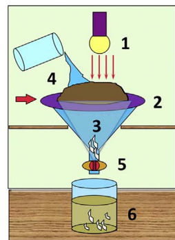
Fig. 2. The two most common devices used for a preliminary survey of soil animals. a) standard dry Berlese funnel extraction; b) wet O'Connor funnel extraction. The use of these extraction methods is sufficient for many basic research and teaching purposes. Nematodes can also be extracted using wet extraction in the dark (no light). More demanding and specific tools are necessary for a more extensive survey of soil pedofauna. In particular, earthworms cannot be extracted with these devices and combinations of hand-sorting and chemical extraction are performed in the field.
