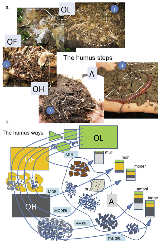
Fig. 30. a) Humus system formation according to four typical steps of litter transformation (OL, OF, OH and A horizons). The time of formation/disappearance of each horizon depends on environmental factors; b) Litter transformation and final humus systems. Numbers and succession of the different horizons are influenced by environmental conditions. Five different points of dynamic equilibrium (called humus interaction systems or humus systems) have been described in this guide for terrestrial ecosystems.
