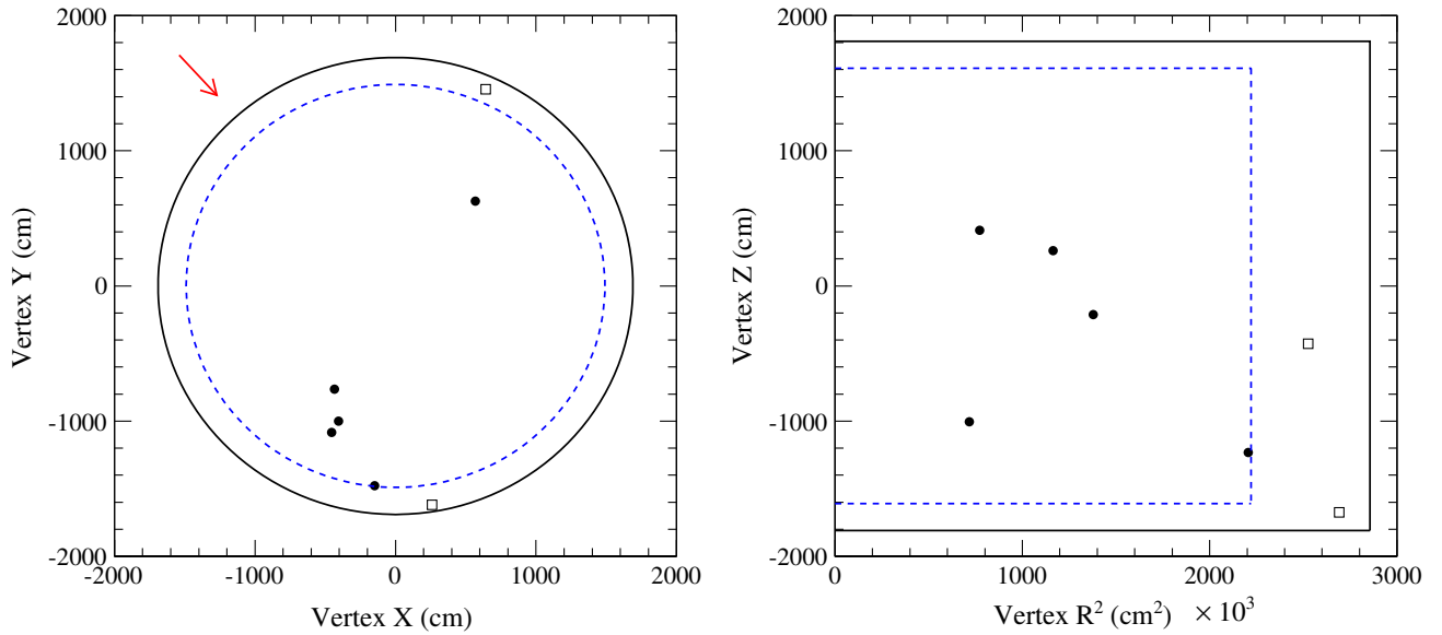
FIG. 26. Two-dimensional vertex distributions of the observed \nu_e \text{CC}1\pi^+ candidate events in (X, Y) and (R^2, Z) . The arrow indicates the neutrino beam direction, and the dashed line indicates the fiducial volume boundary. Events indicated by open square markers passed all of the \nu_e \text{CC}1\pi^+ selection cuts except for the fiducial volume cut.
