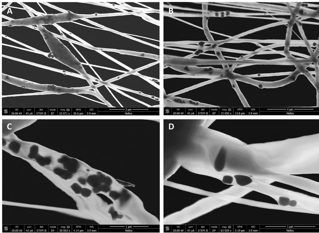
Fig. 5. STEM micrographs of BTNP/PVDF 10/90 electrospun fibers obtained with a collector tangential velocity of 3.7 \text{ m}\cdot\text{s}^{-1} at different magnifications in the range of 10,000\times to 65,000\times . (A, B) dispersion of BTNPs inside the electrospun fibers; (A) beads induced by the presence of BTNP aggregates; (C) BTNP aggregates inside an electrospun fiber; and (D) BTNP dispersed inside an electrospun fiber.
