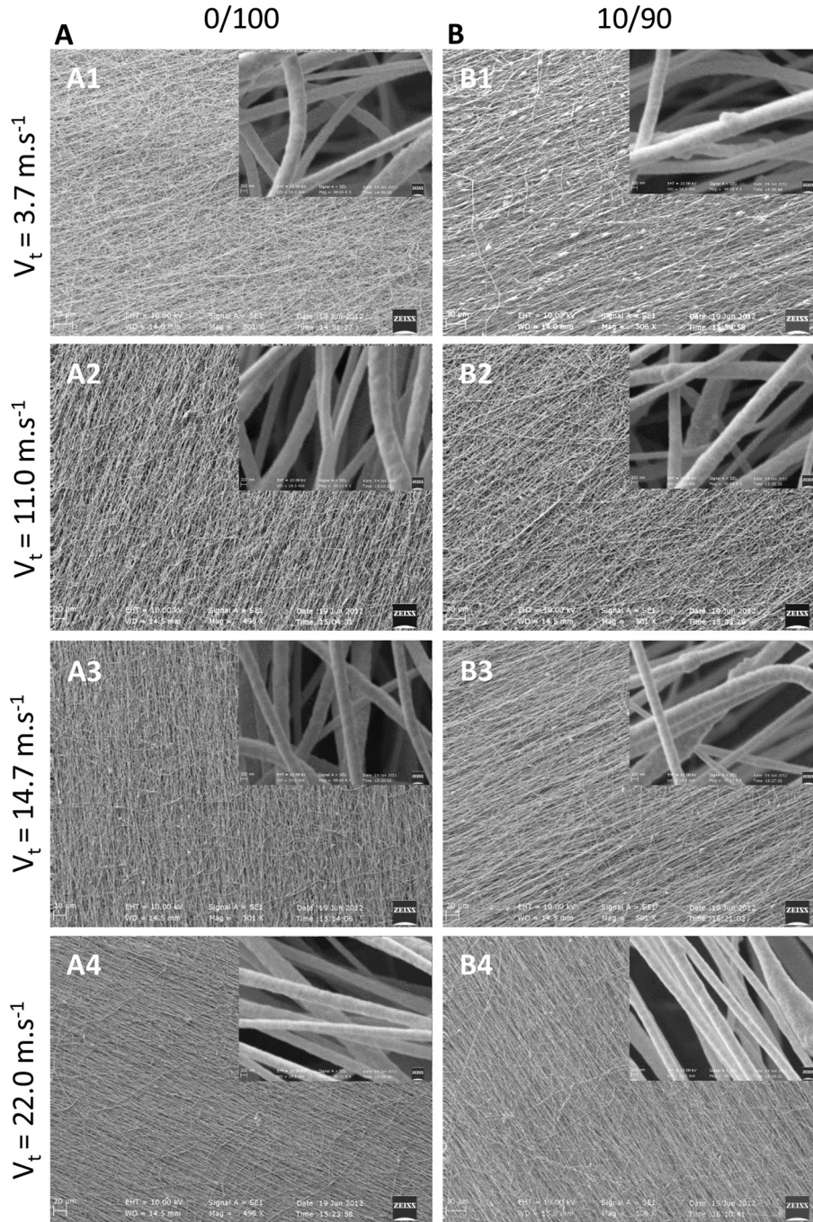
Fig. 3. Morphology of BTNP/PVDF electrospun fibers collected on a rotating disk at different tangential velocities in the range of 3.7 to 22.0 \text{m}\cdot\text{s}^{-1} ; (A) 0/100 and (B) 10/90 w/w compositions.
