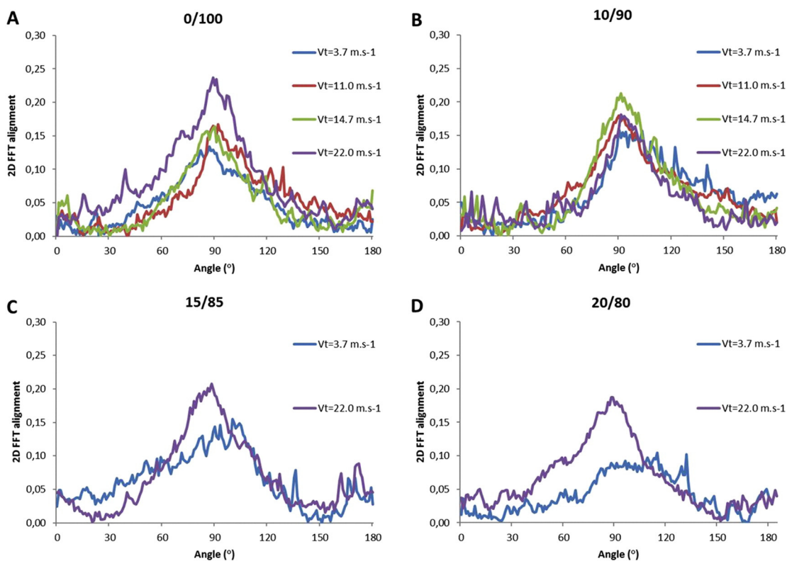
Fig. 7. Two-dimensional FFT plots of fibers collected at different tangential velocities for the following BTNP/PVDF weight compositions: (A) 0/100; (B) 10/90; (C) 15/85; and (D) 20/80.
