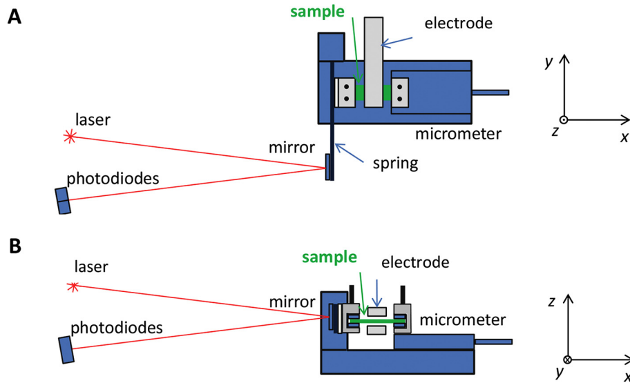
Fig. 2. Schematic of the setup used to measure the converse piezoelectric effect, (A) top view and (B) side view.
