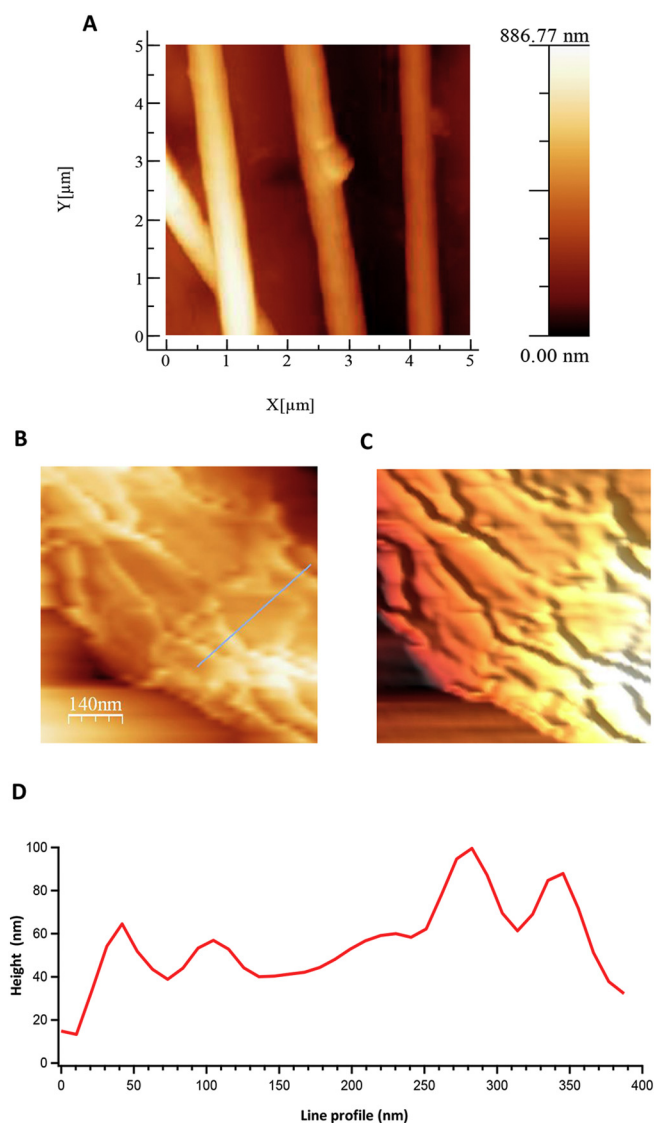
Fig. 6. Topographical analysis of BTNP/PVDF fibers. (A) A representative tapping mode AFM micrograph showing the surface topography of the fibers and a BTNP emerging from the polymer; (B–C) Representative results of SNOM analysis: (B) Surface topography of the fiber showing nanowrinkles, (C) Pseudo 3D reconstruction, and (D) fiber profile along the blue line in (B). (For interpretation of the references to colour in this figure legend, the reader is referred to the web version of this article.)
