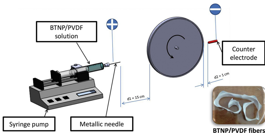
Fig. 1. Scheme of the electrospinning apparatus used to produce the BTNP/PVDF fibers, with weight compositions 0/100, 10/90, 15/85 and 20/80.
