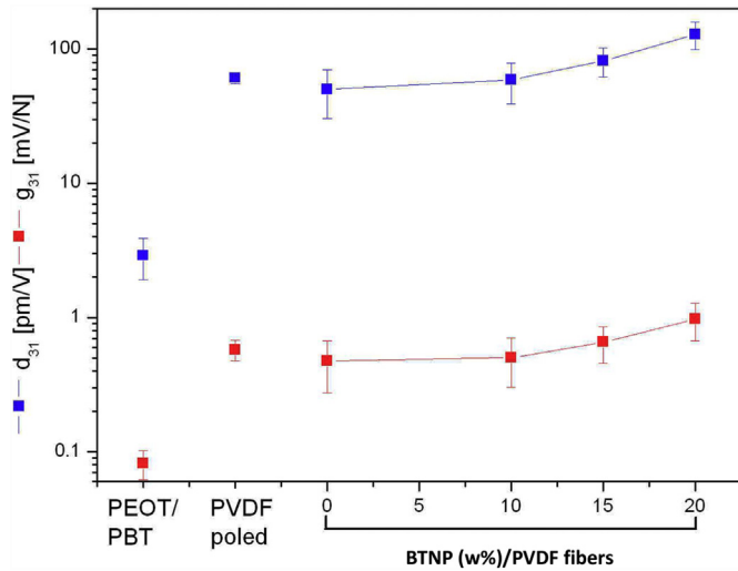
Fig. 10. Graph showing the values of the piezoelectric coefficients for the different materials tested: PEOT/PBT random fiber mesh (negative test), PVDF from Goodfellow (positive test), and the four different weight compositions of electrospun BTNP/PVDF fibers.
