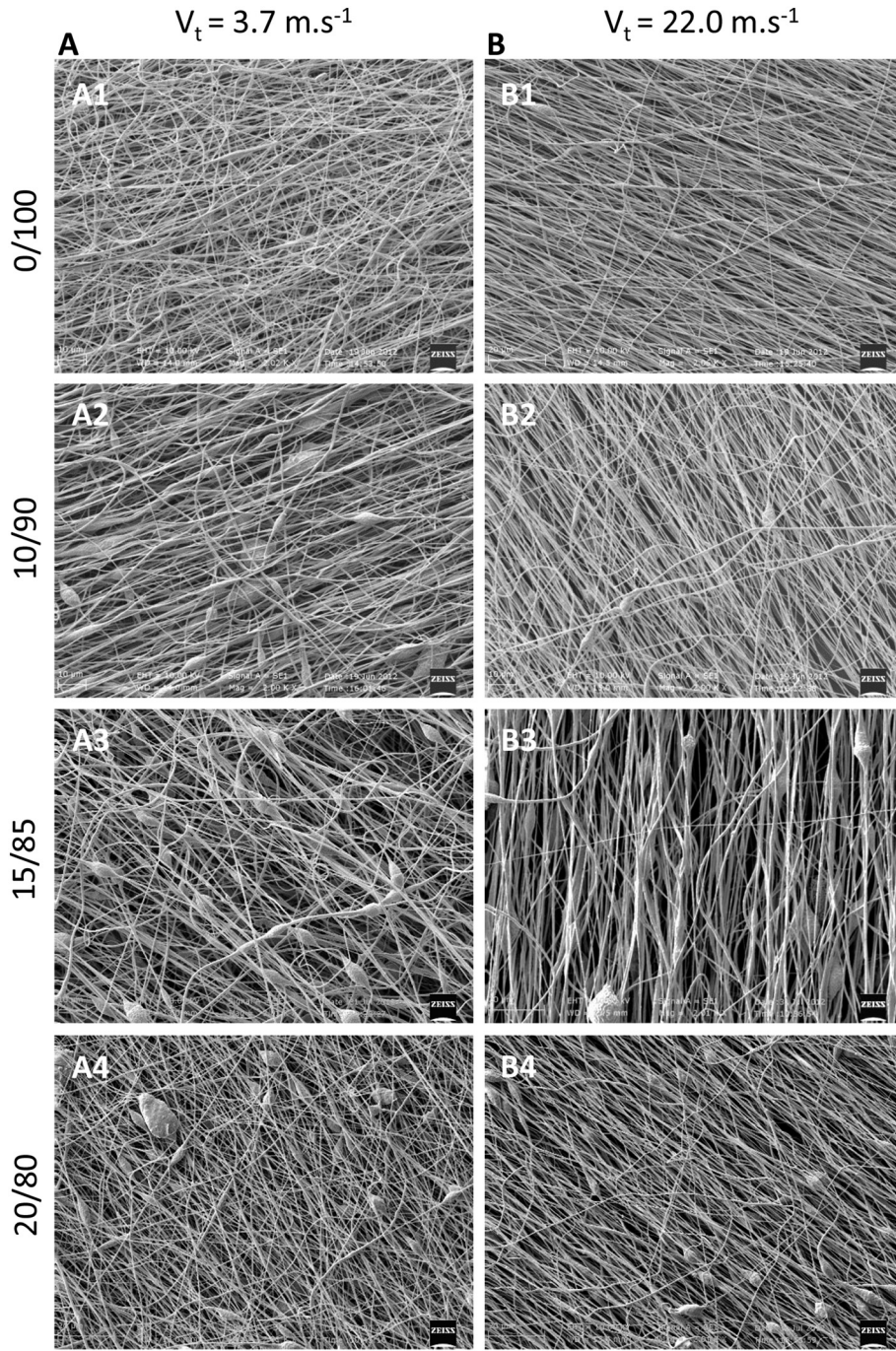
Fig. 4. Morphology of BTNP/PVDF electrospun fibers of different weight compositions, in the range of 0/100 to 20/80, collected on a rotating disk at low and high tangential velocity; (A) 3.7 \text{ m}\cdot\text{s}^{-1} and (B) 22.0 \text{ m}\cdot\text{s}^{-1} .
