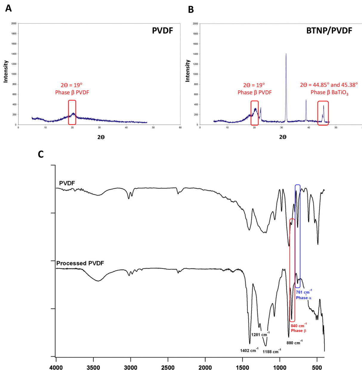
Fig. 8. Characterization of crystalline phases. (A, B) XRD analysis showing the 2\theta peaks in BTNP/PVDF fibers corresponding to the piezoelectric \beta phases of PVDF and BaTiO 3 : (A) 0/100 and (B) 20/80 weight compositions. (C) ATR-FTIR analysis showing the peak intensity of the non-piezoelectric \alpha phase and the piezoelectric \beta phase in the raw PVDF and the electrospun PVDF fibers.
