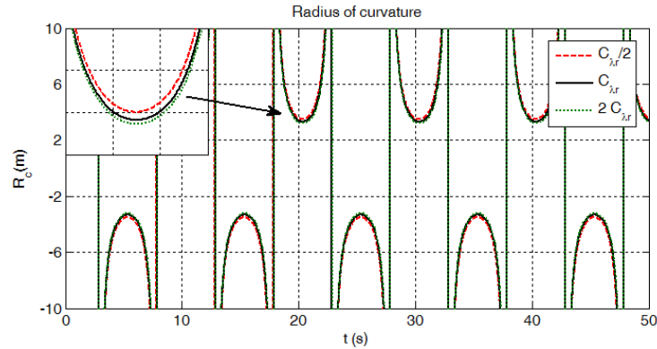
Fig. (14). Effect of cornering stiffness on slalom curvature radius.
