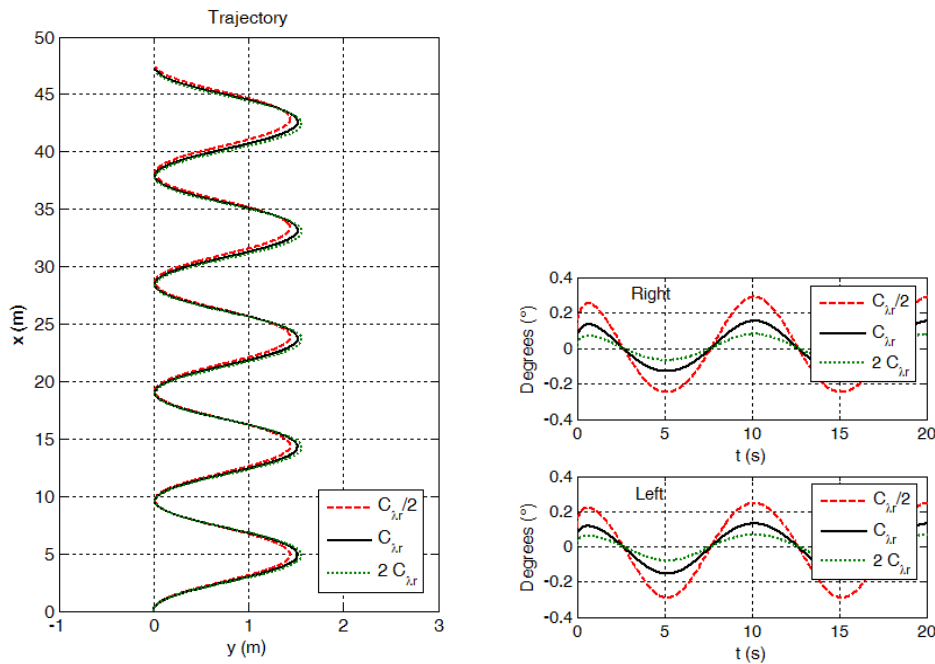
Fig. (13). Effect of cornering stiffness on slalom trajectory of CM and side slip angles.
