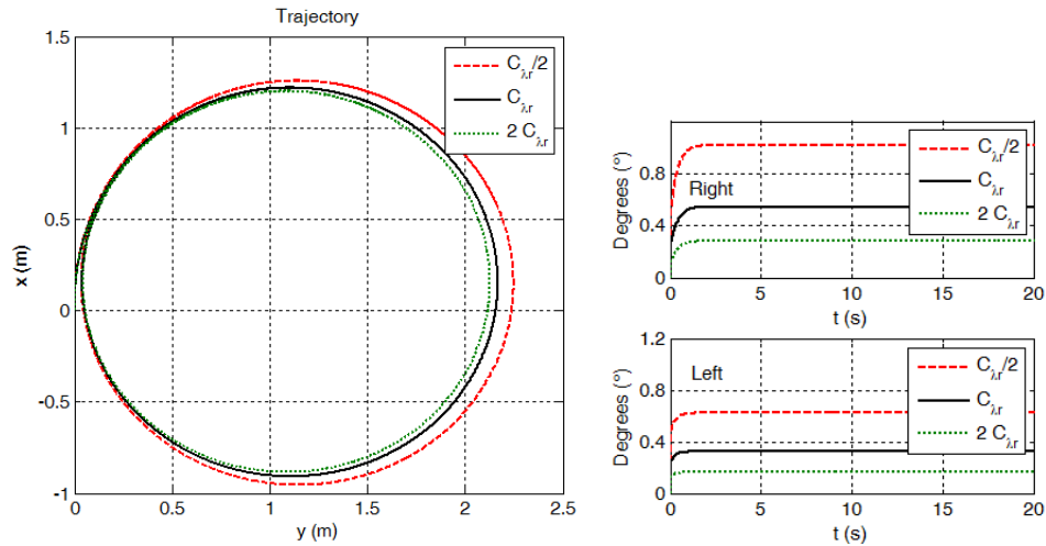
Fig. (12). Effect of cornering stiffness on steady turning trajectory of CM and side slip angles.
