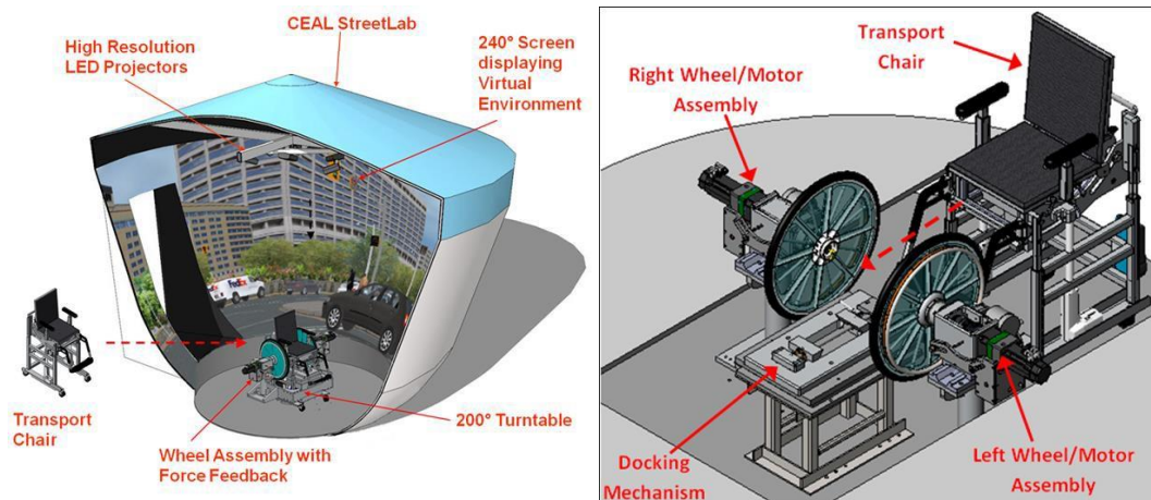
Fig. (1). Design of the wheelchair simulator using the StreetLab virtual environment.
