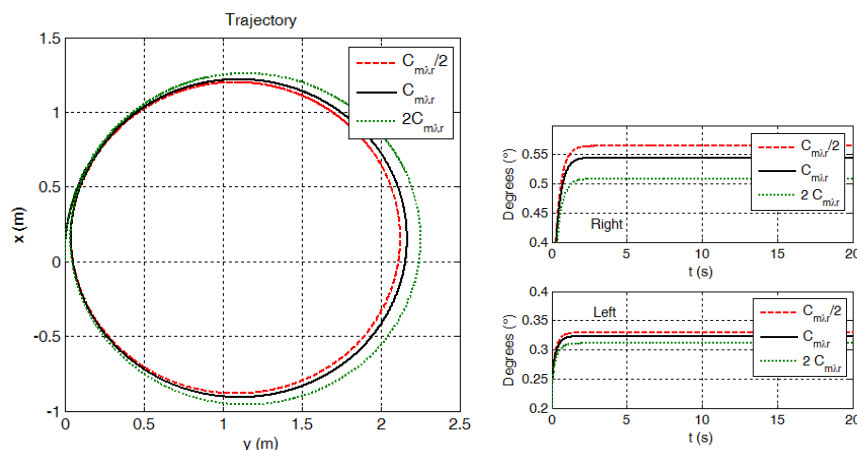
Fig. (15). Effect of self aligning torque on steady turning trajectory of CM and side slip angles.
