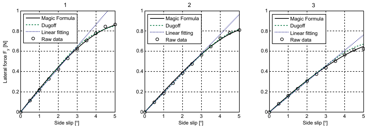
Fig. (8). Fittings of lateral force raw data by means of the Magic Formula and Dugoff models for tire A; (1) reference condition, (2) decreased inflation pressure, (3) increased load.
