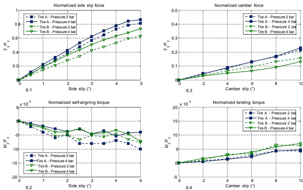
Fig. (6). Effect of inflation pressure on tire forces and torques.
