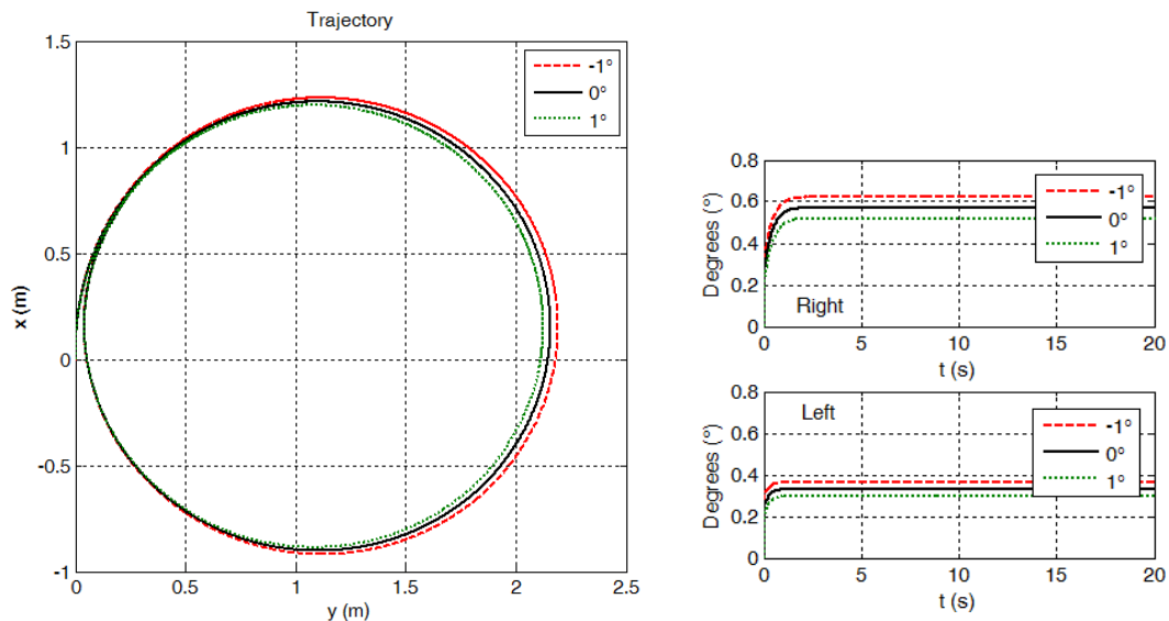
Fig. (18). Effect of camber angle on steady turning trajectory of CM and side slip angles.
