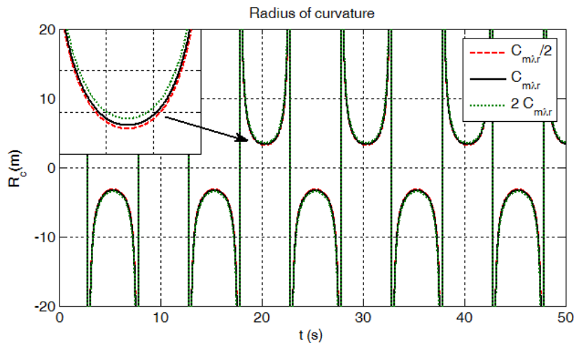
Fig. (17). Effect of self-aligning torque on slalom curvature radius.
