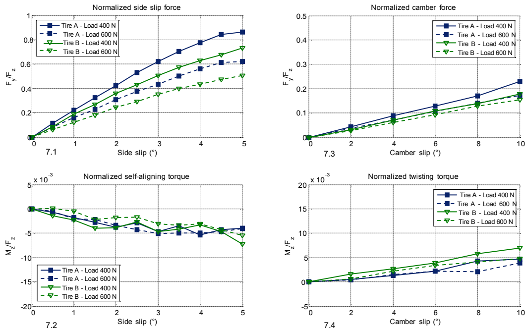
Fig. (7). Effect of vertical load on tire forces and torques.
