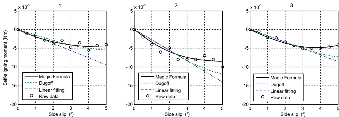
Fig. (9). Fittings of self-aligning moment raw data by means of the Magic Formula and Dugoff models for tire A; (1) reference condition, (2) decreased inflation pressure, (3) increased load.
