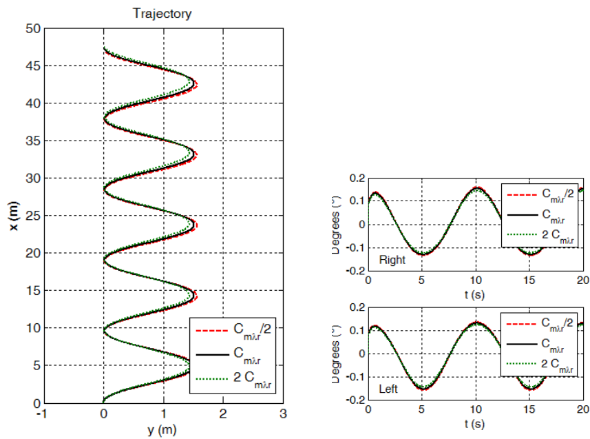
Fig. (16). Effect of self-aligning torque on slalom trajectory of CM and side slip angles.
