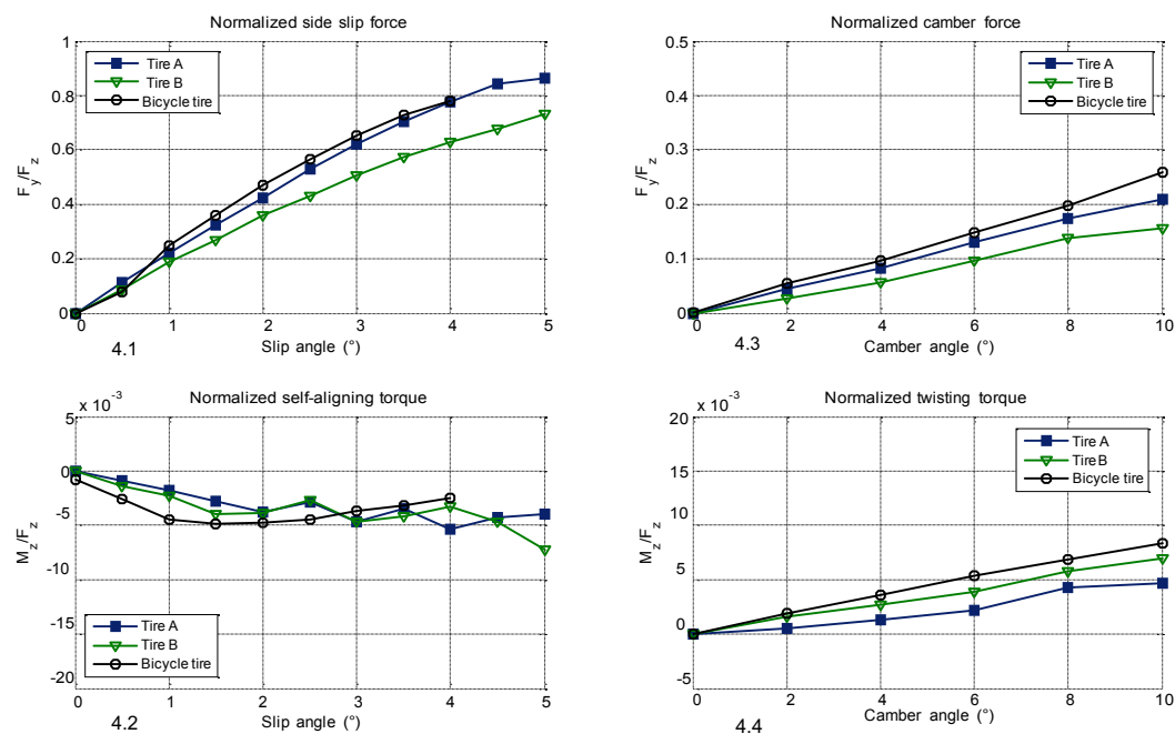
Fig. (4). Forces and torques of wheelchair and bicycle tires in reference conditions (vertical load 400 N, inflation pressure 4 bar and disc speed 4 km/h).
