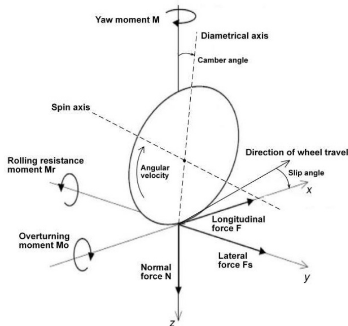
Fig. (3). The coordinate system for the definition of tire forces and torques.
