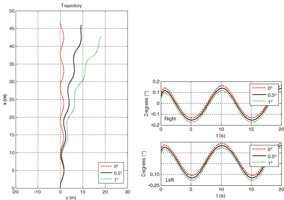
Fig. (19). Effect of camber angle on slalom trajectory of CM and side slip angles.
