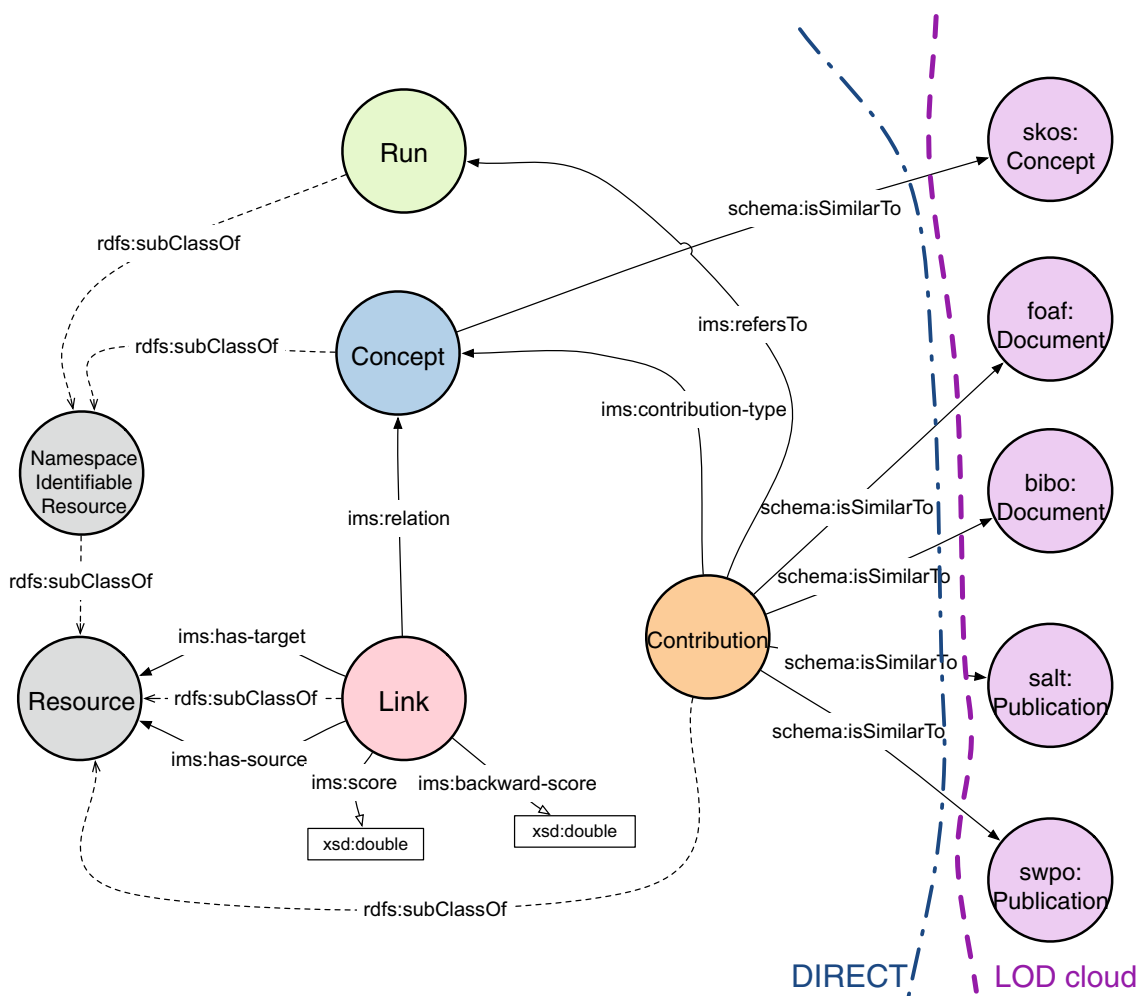
Fig. 5 The scientific production area classes and properties
