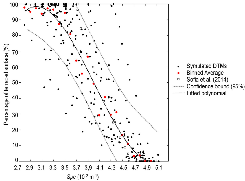
Fig. 6. Spc for the simulated DTMs, the binned average values and the derived curve fitting, as compared to the Spc for the Mediterranean dataset (Sofia et al., 2014). The 95% confidence interval is also shown.
