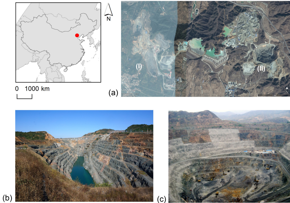
Fig. 2. Location map of the Miyun Iron Mine (a) and pictures of the two analysed iron open-pit mines (Beijing District, P.R. China): mine I (b) and mine II (c).
