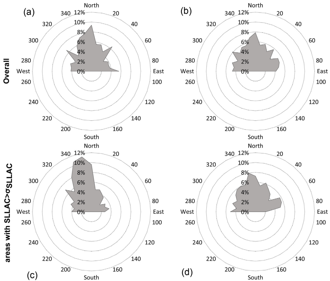
Fig. 10. Radar graphs of the orientation of the correlation lengths for the two mining sites, considering the overall SLLAC maps (a and b), and only those areas having a correlation length greater than one standard deviation of the SLLAC (c and d).
