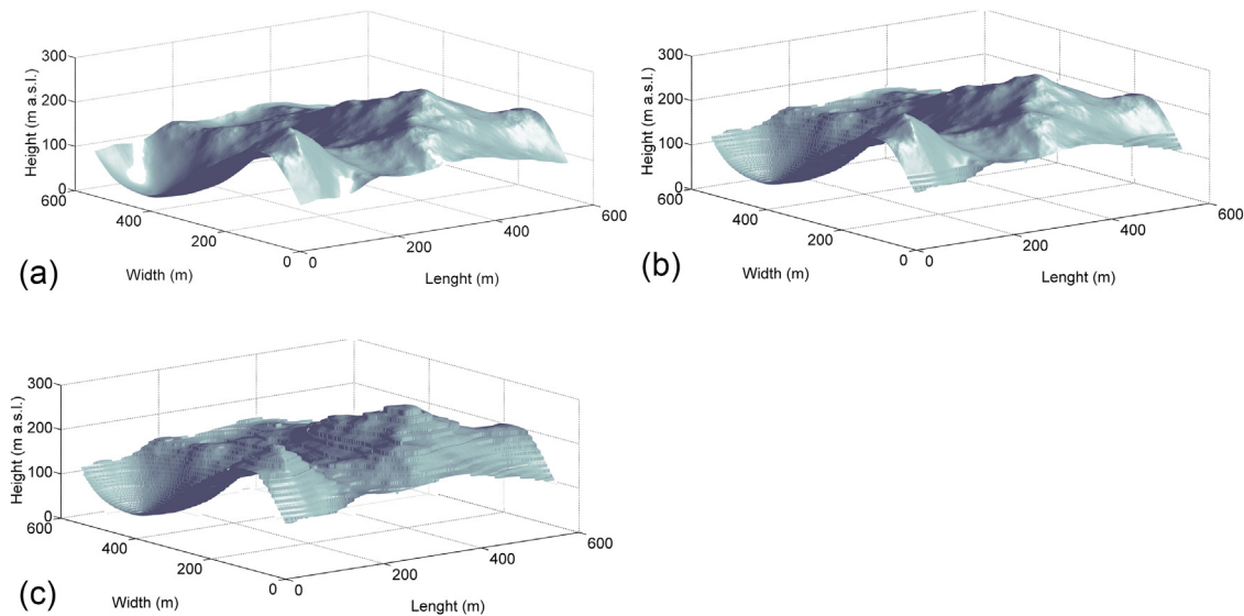
Fig. 5. (a) An example of a synthetic DTM. The same DTM having terraces covering (b) 50% and (c) 100% of the area.
