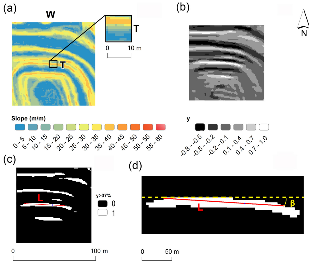
Fig. 4. Example of the calculation of SLLAC for a single moving window (W). (a) For each moving window (W), a slope template T is identified, having the centre at the centre of W. The cross-correlation between T and W is computed (b). The resulting map is thresholded at 37% of its maximum value (c). The length of correlation is then the length of the longest line passing through the central pixel (blue dot) and connecting two boundary pixels in the extracted area connected to the central pixel. (d) Measurement of the length orientation \beta (in this example, it is about -10^\circ ).
