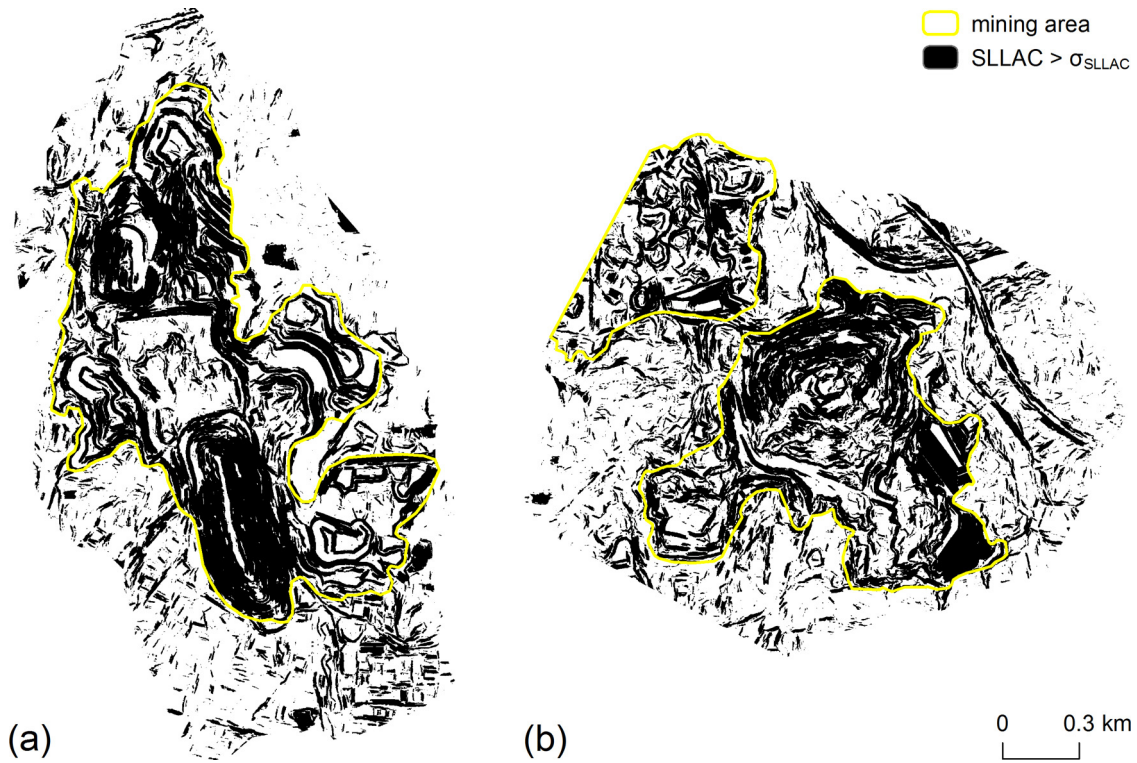
Fig. 9. Areas having correlation lengths larger than one standard deviation of SLLAC (a and b). The yellow boundaries represent the extraction areas where terraces are present.
