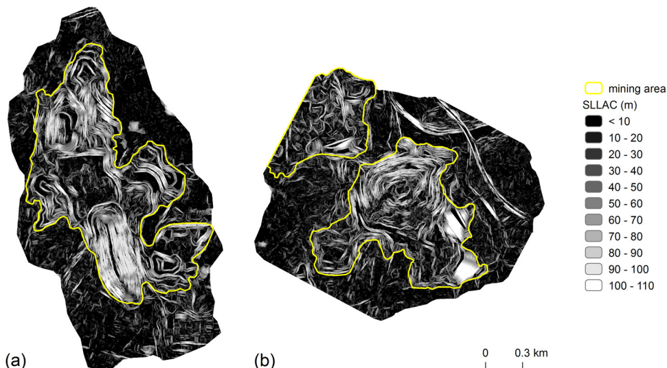
Fig. 7. SLLAC maps for mining sites I and II (a and b). The yellow boundaries represent the extent of the extraction areas within the mine sites.
