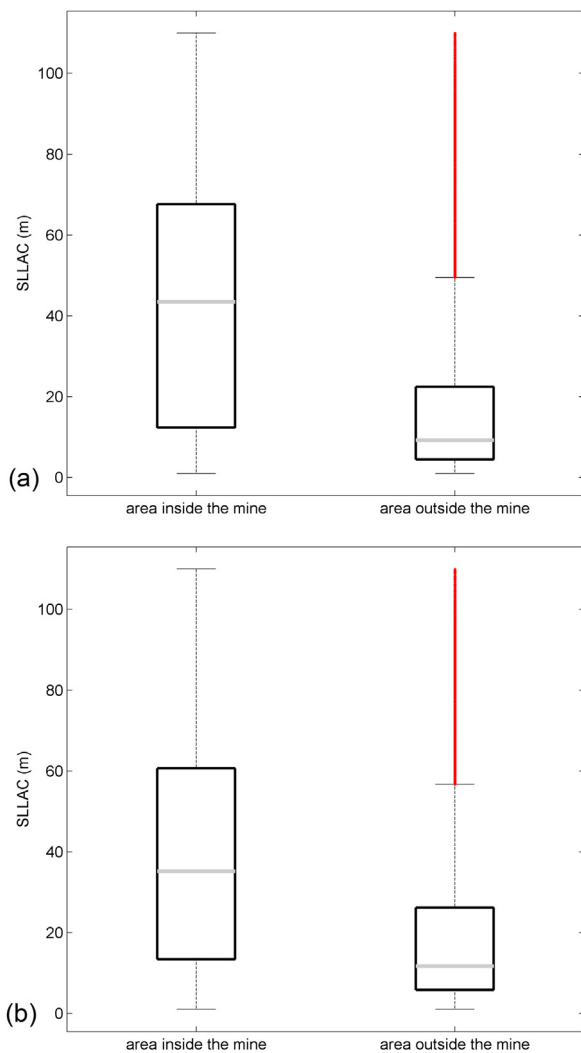
Fig. 8. A boxplot of the SLLAC values considering the extraction areas (highlighted in yellow in Fig. 7) as compared to the surroundings. (a) and (b) in the figure correspond to mining site I and II.
